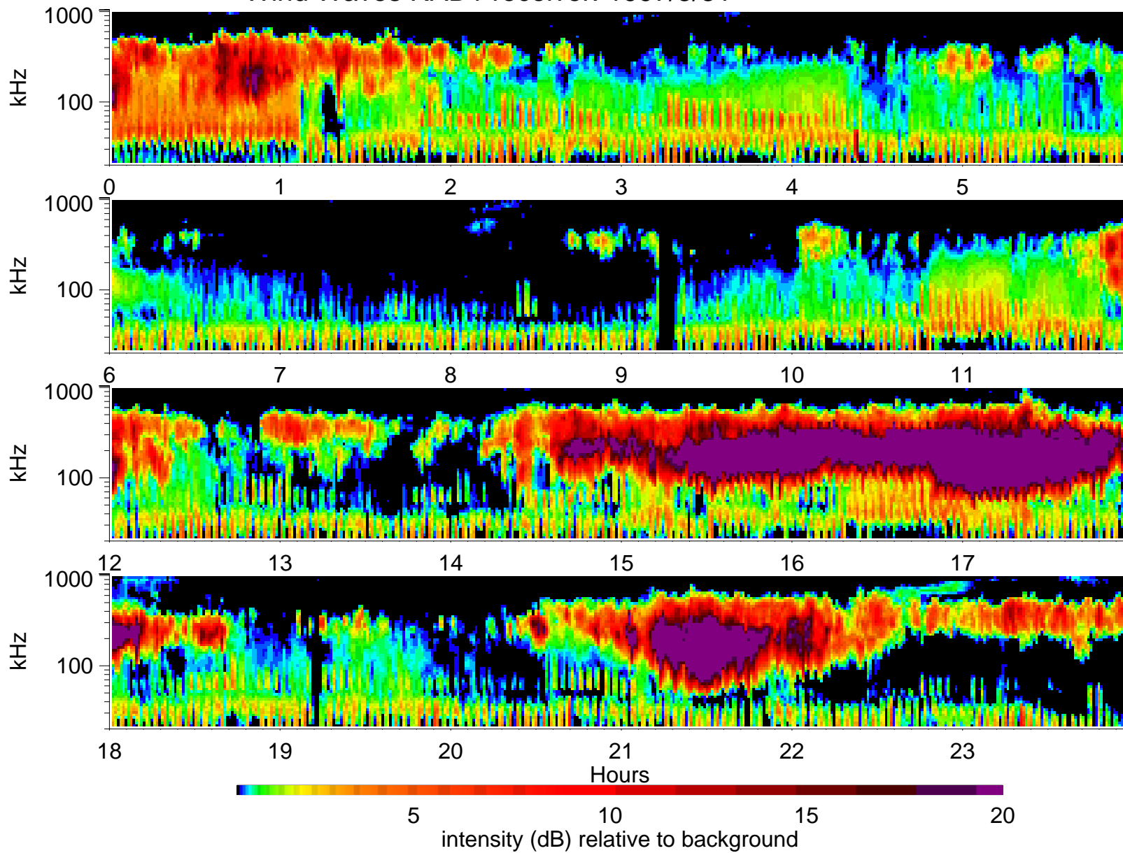
Wind Waves RAD1 receiver: 1997/5/31
