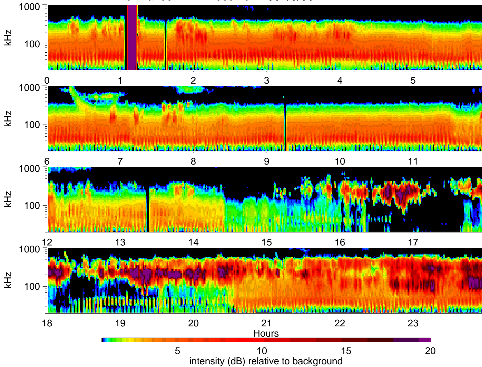
Wind Waves RAD1 receiver: 1997/5/30
