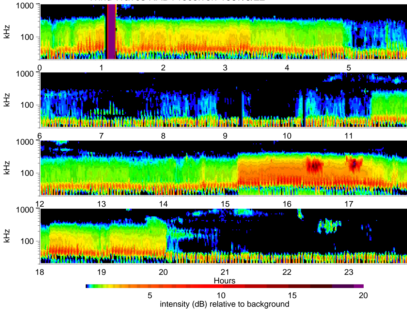
Wind Waves RAD1 receiver: 1997/5/22
