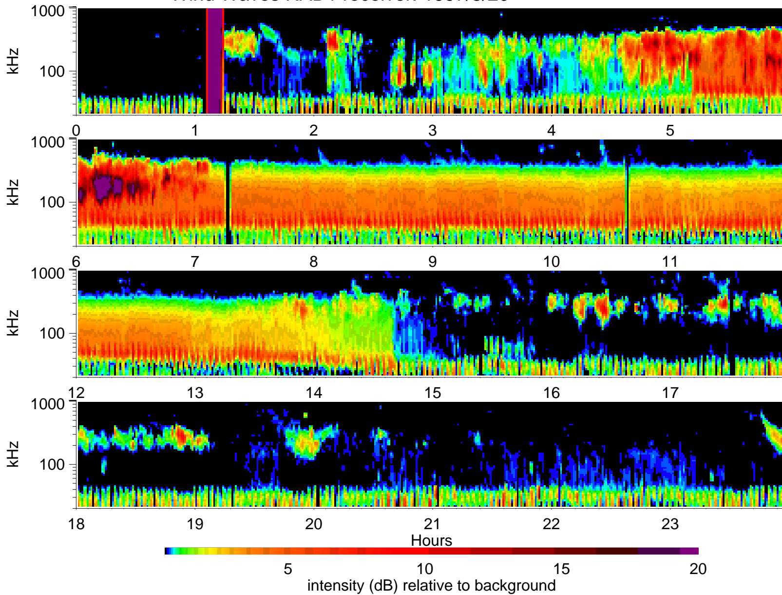
Wind Waves RAD1 receiver: 1997/5/20
