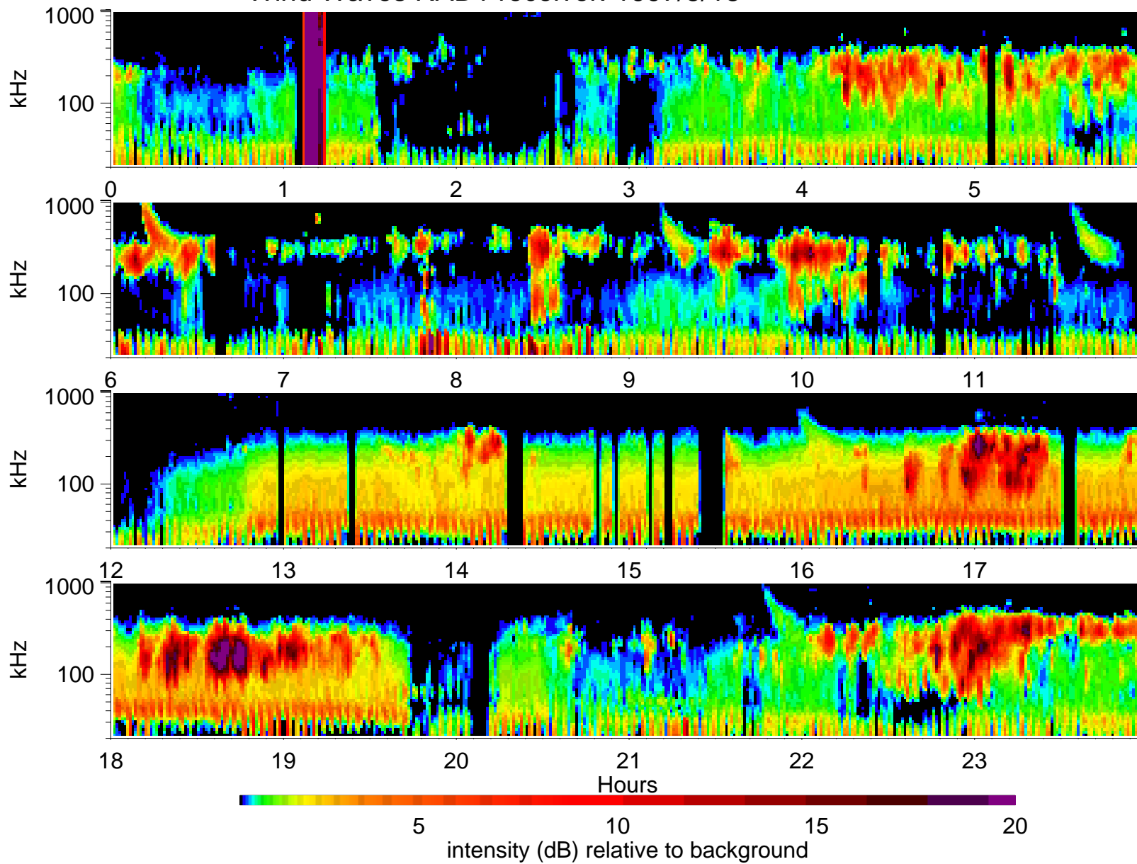
Wind Waves RAD1 receiver: 1997/5/18
