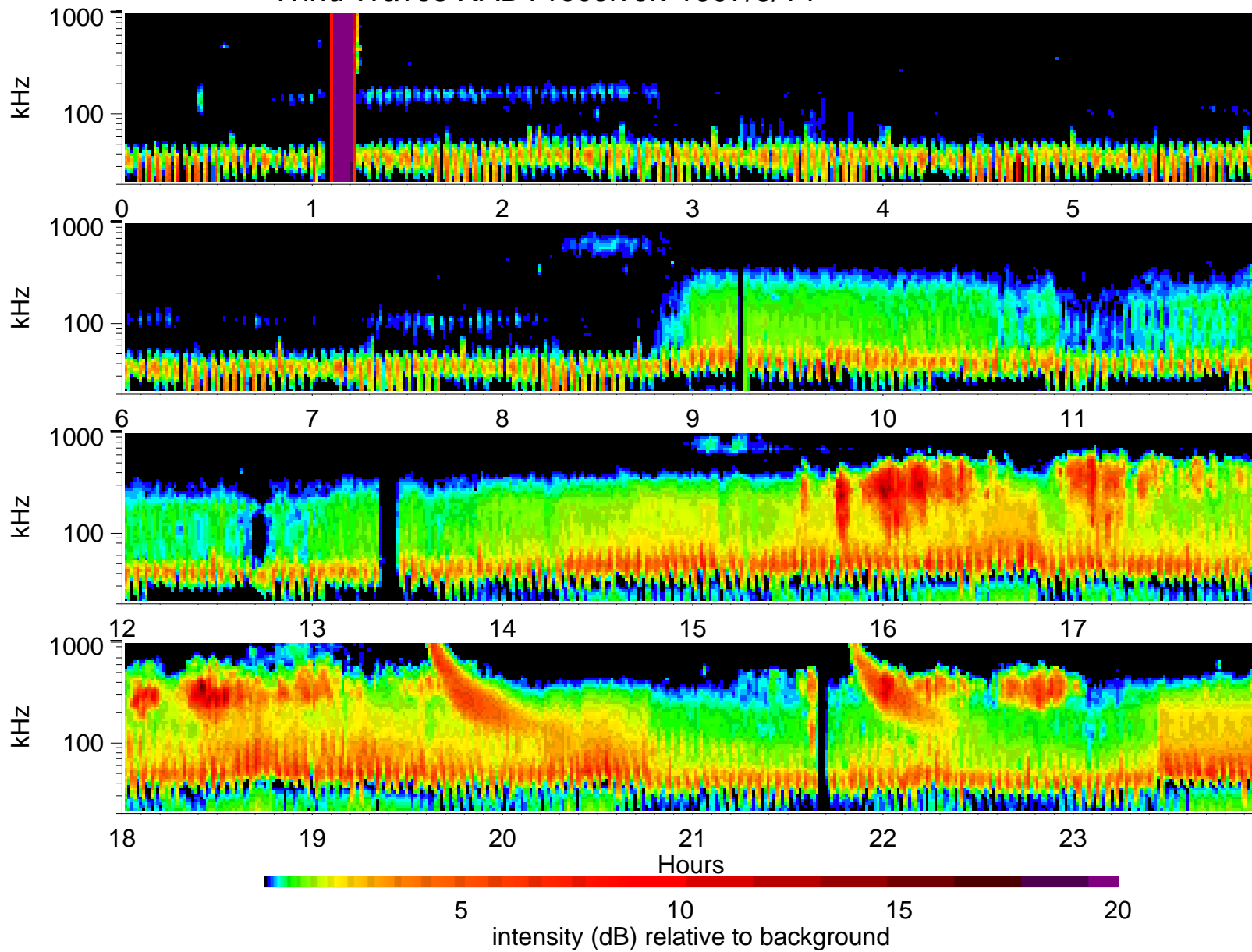
Wind Waves RAD1 receiver: 1997/5/14
