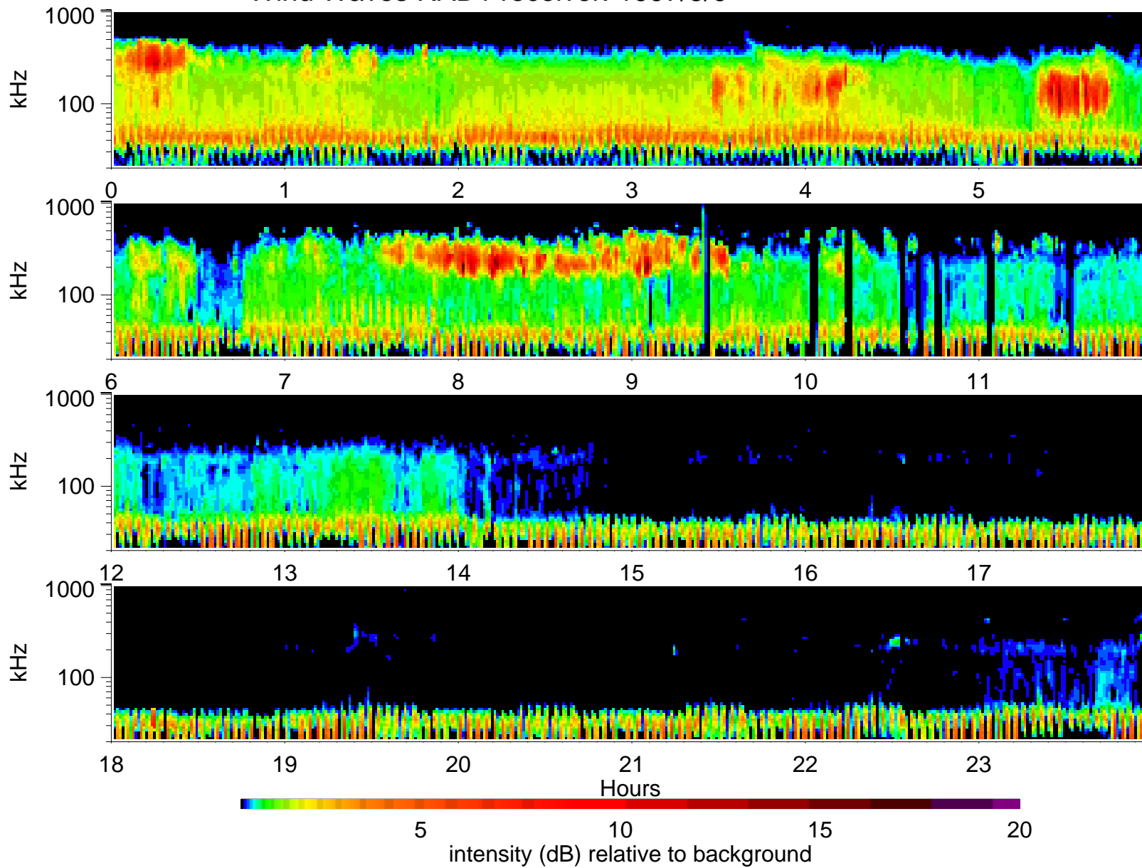
Wind Waves RAD1 receiver: 1997/5/9
