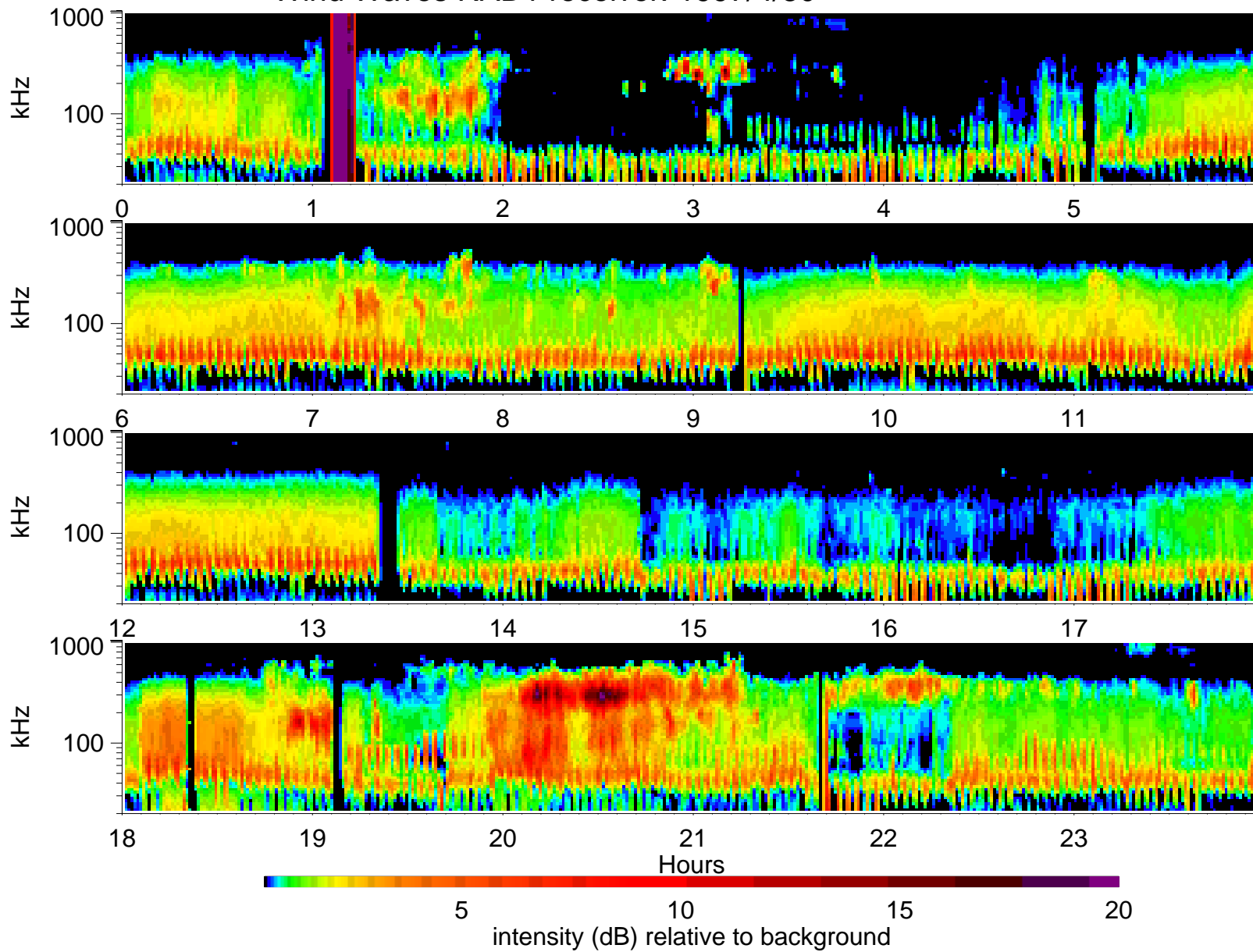
Wind Waves RAD1 receiver: 1997/4/30
