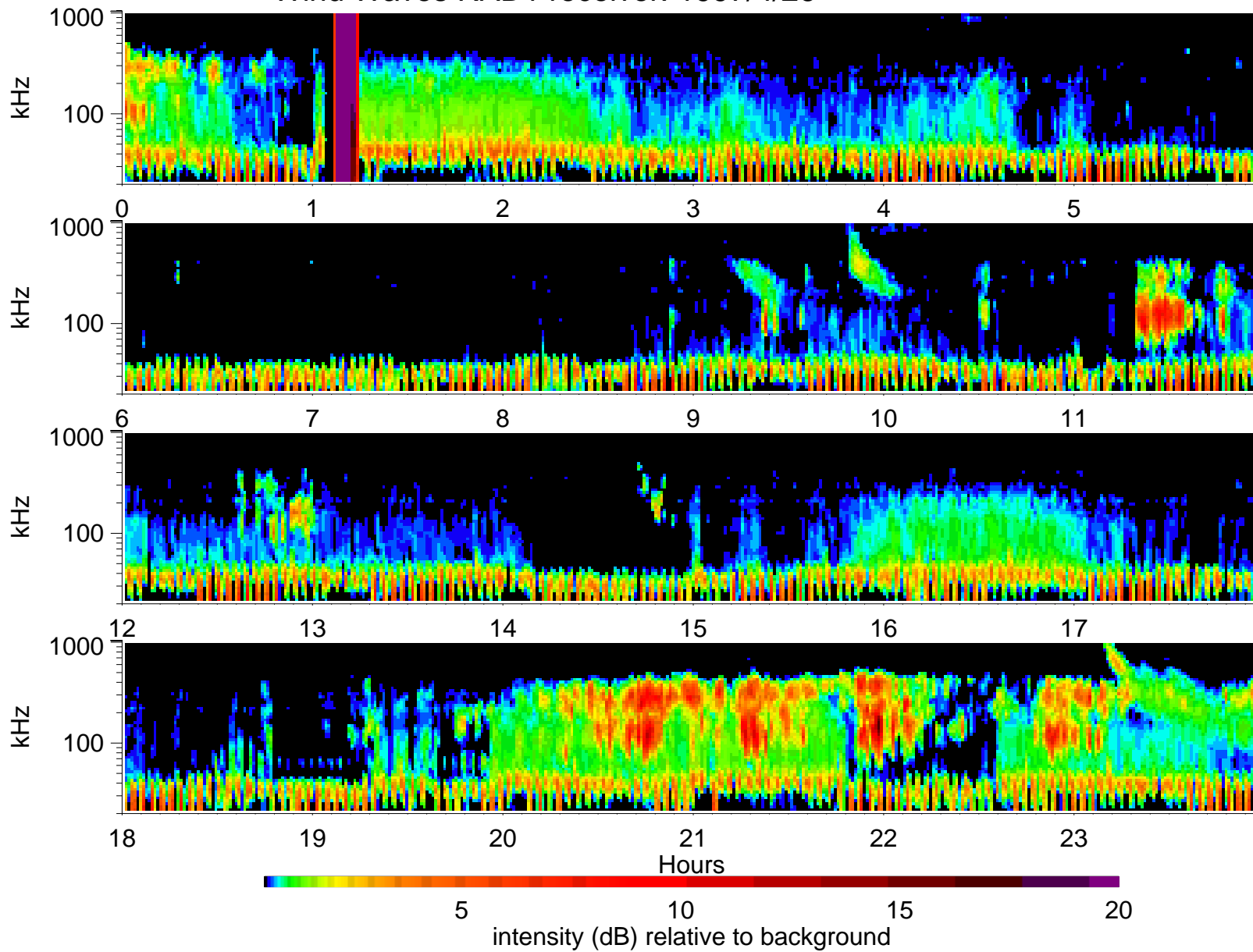
Wind Waves RAD1 receiver: 1997/4/26
