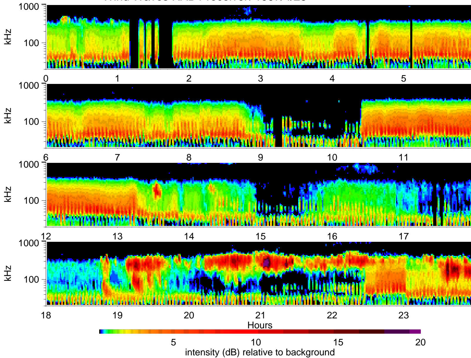
Wind Waves RAD1 receiver: 1997/4/23
