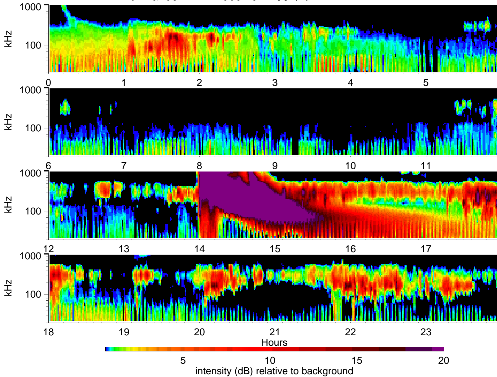
Wind Waves RAD1 receiver: 1997/4/7
