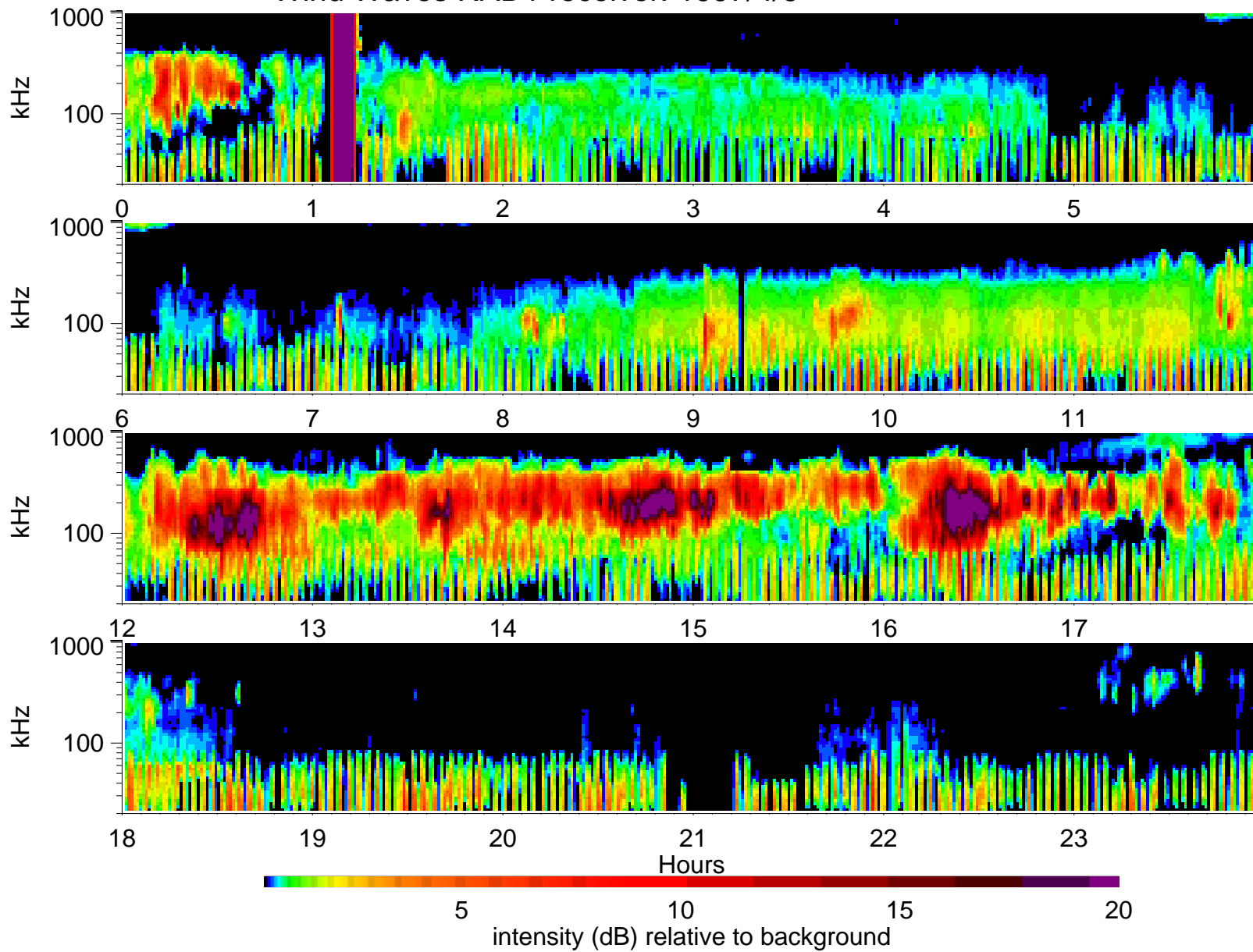
Wind Waves RAD1 receiver: 1997/4/6
