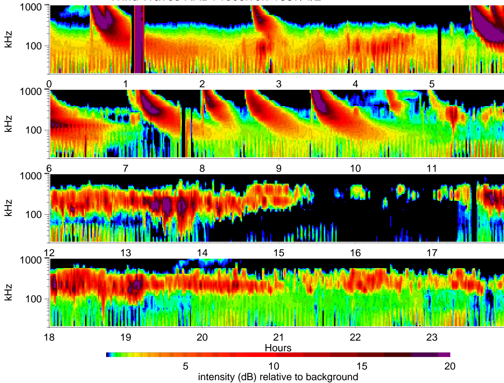
Wind Waves RAD1 receiver: 1997/4/2
