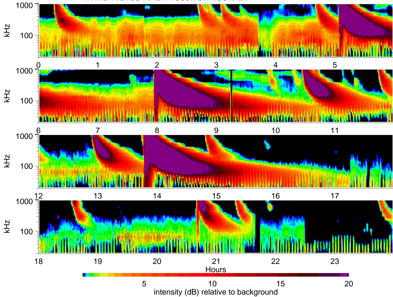
Wind Waves RAD1 receiver: 1997/4/1
