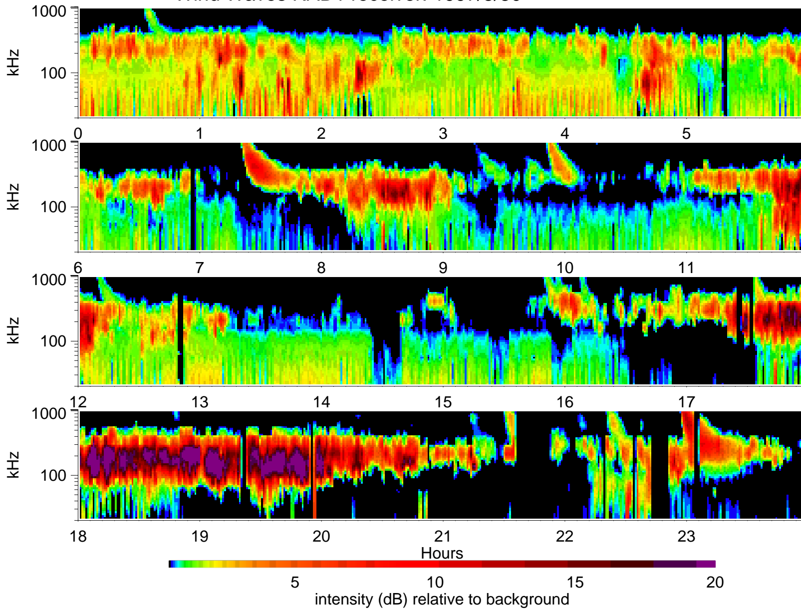
Wind Waves RAD1 receiver: 1997/3/30
