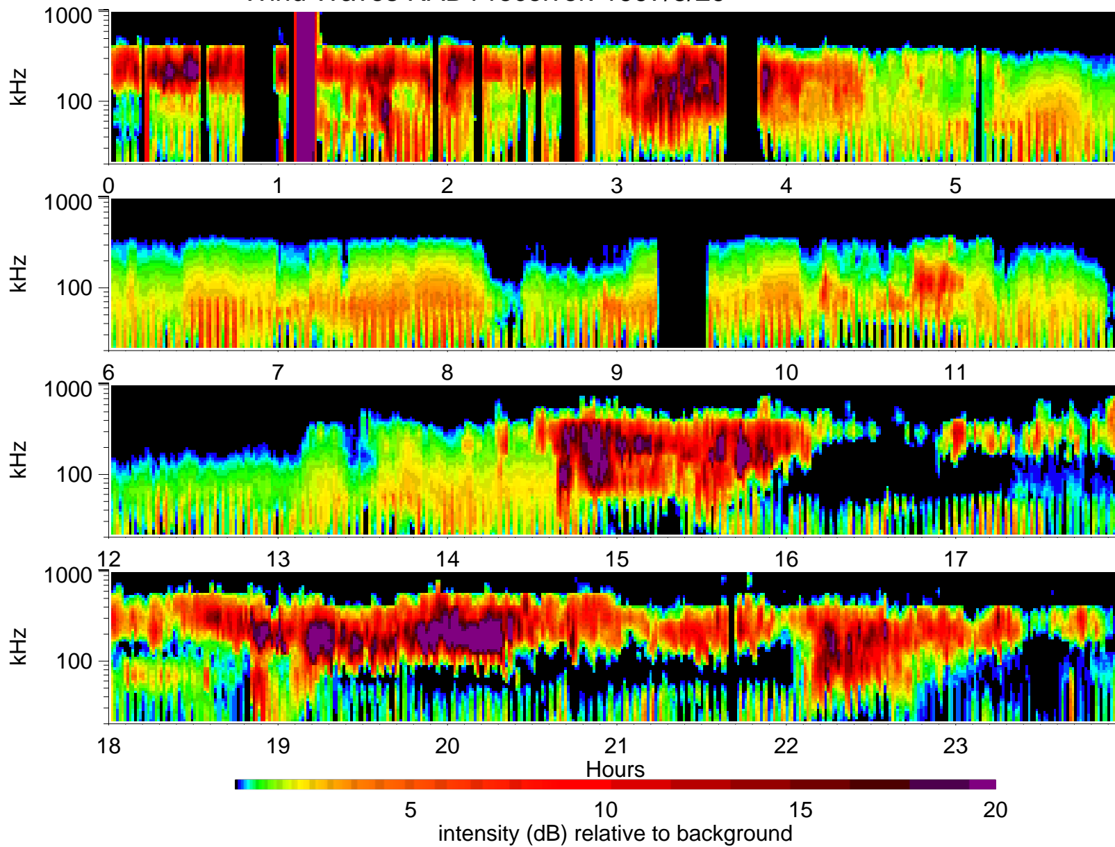
Wind Waves RAD1 receiver: 1997/3/29
