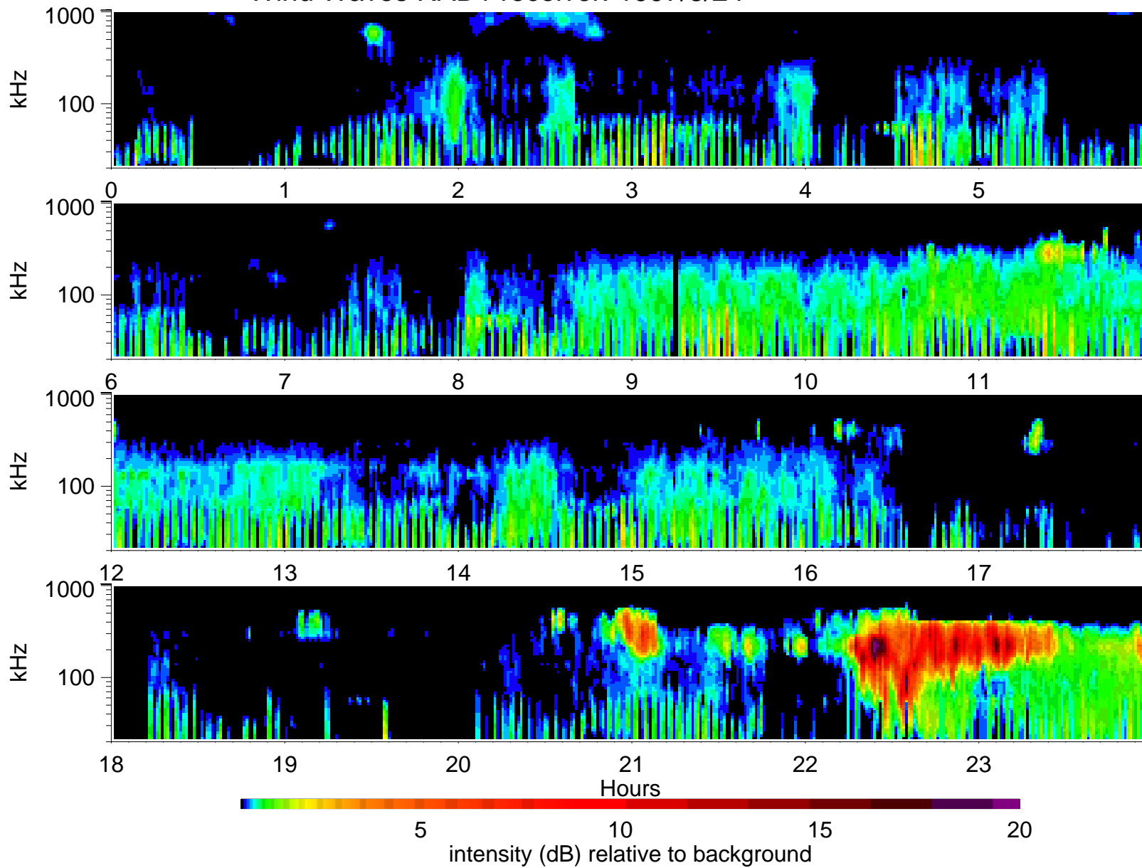
Wind Waves RAD1 receiver: 1997/3/24
