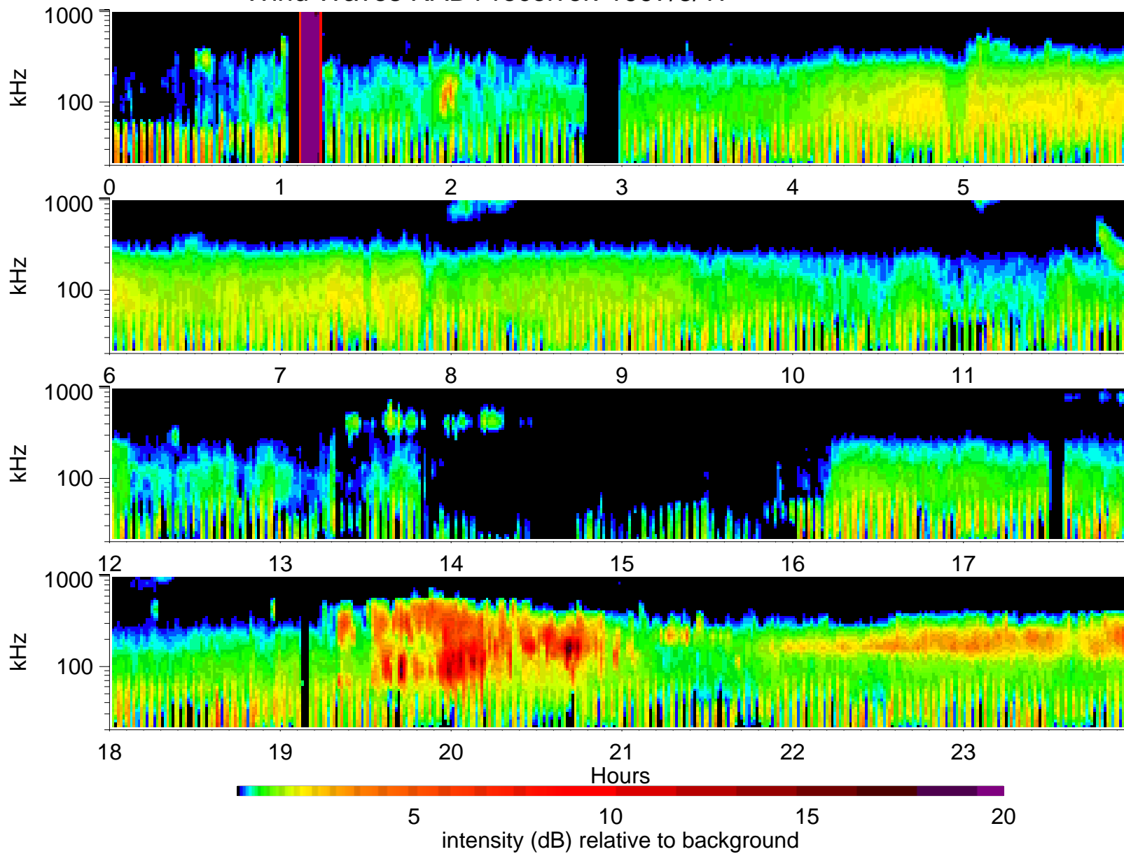
Wind Waves RAD1 receiver: 1997/3/17
