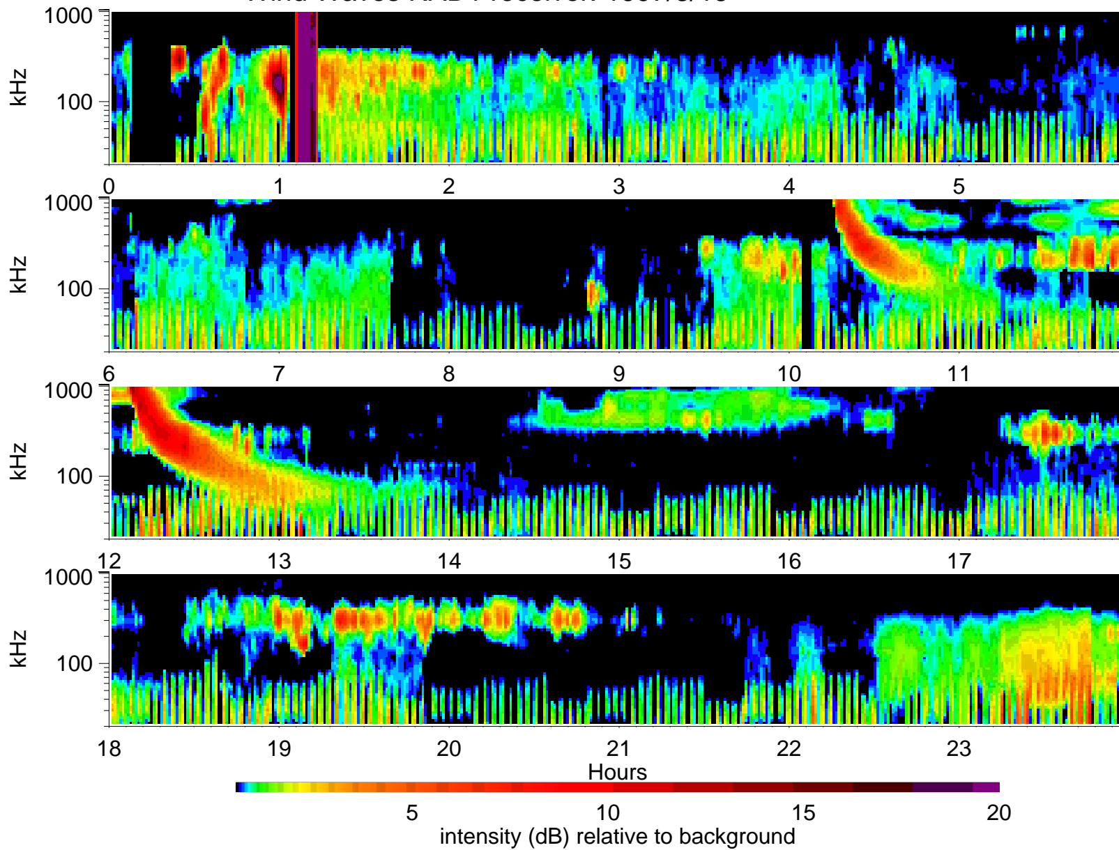
Wind Waves RAD1 receiver: 1997/3/15
