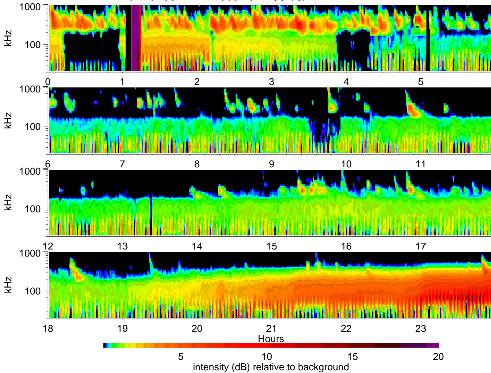
Wind Waves RAD1 receiver: 1997/3/11
