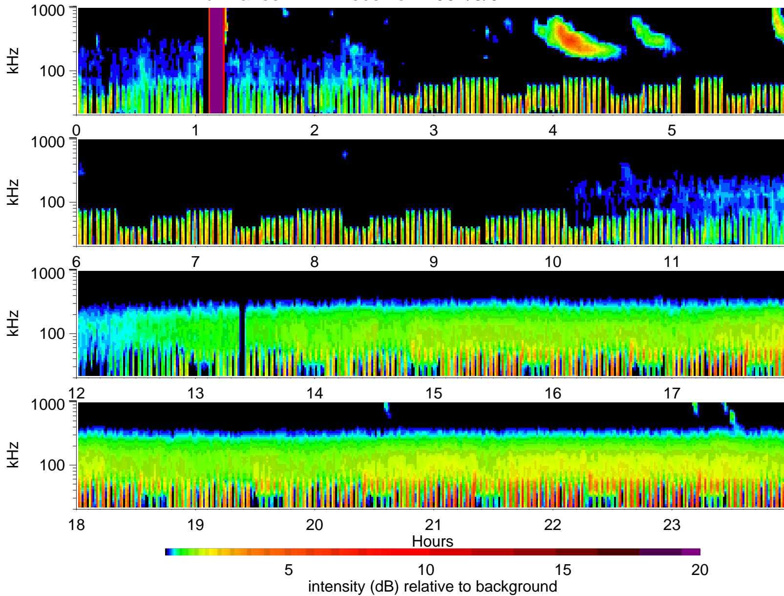
Wind Waves RAD1 receiver: 1997/3/9
