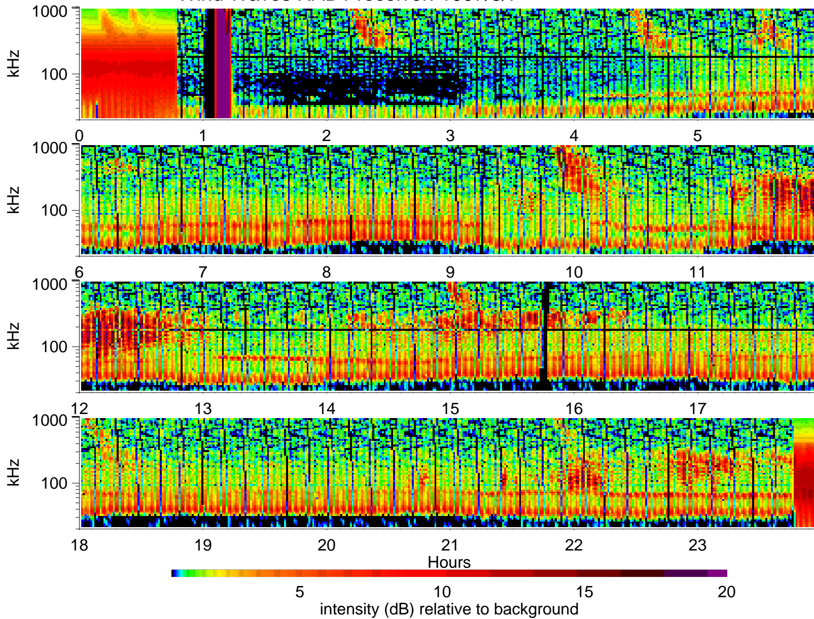
Wind Waves RAD1 receiver: 1997/3/7
