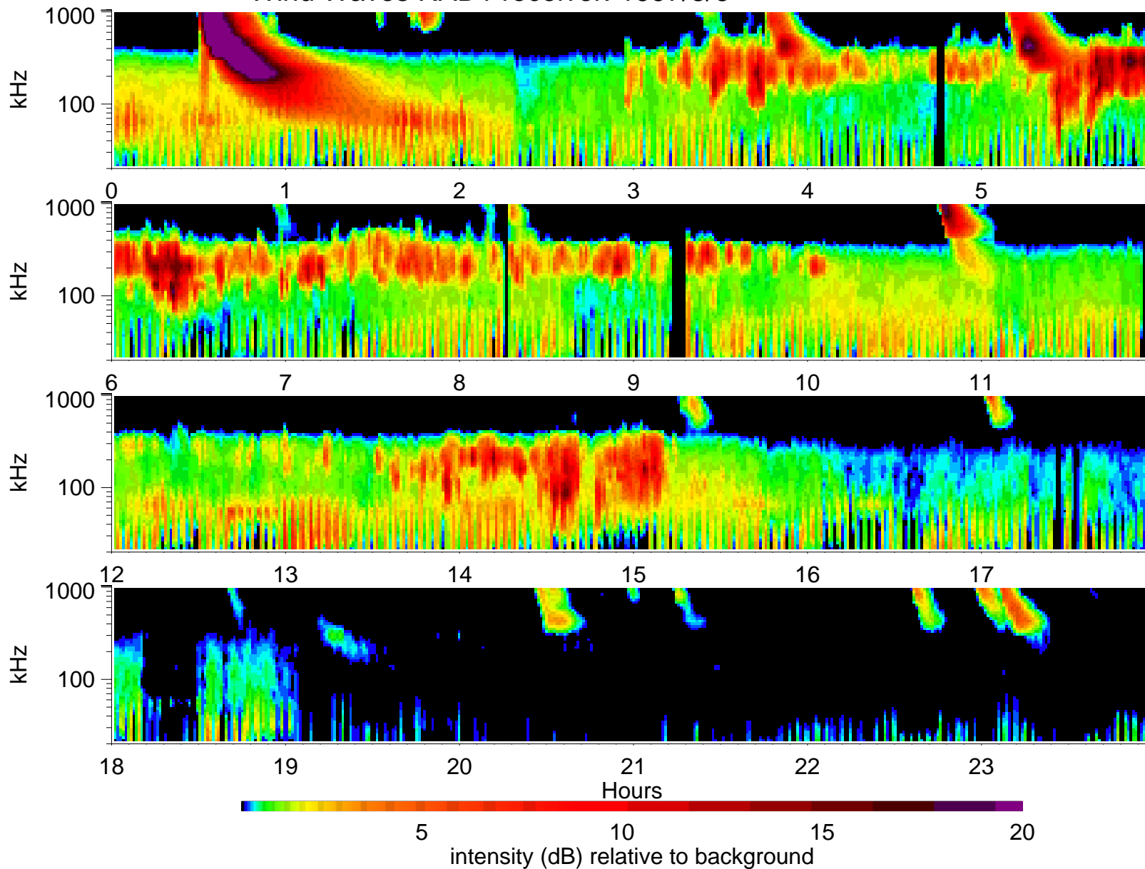
Wind Waves RAD1 receiver: 1997/3/6
