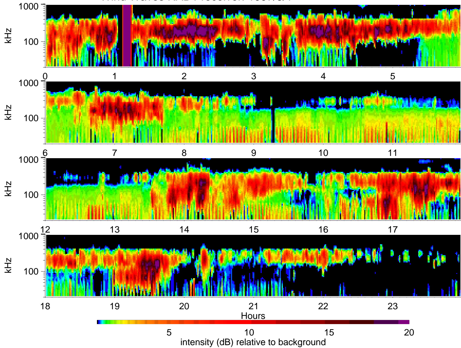
Wind Waves RAD1 receiver: 1997/3/1
