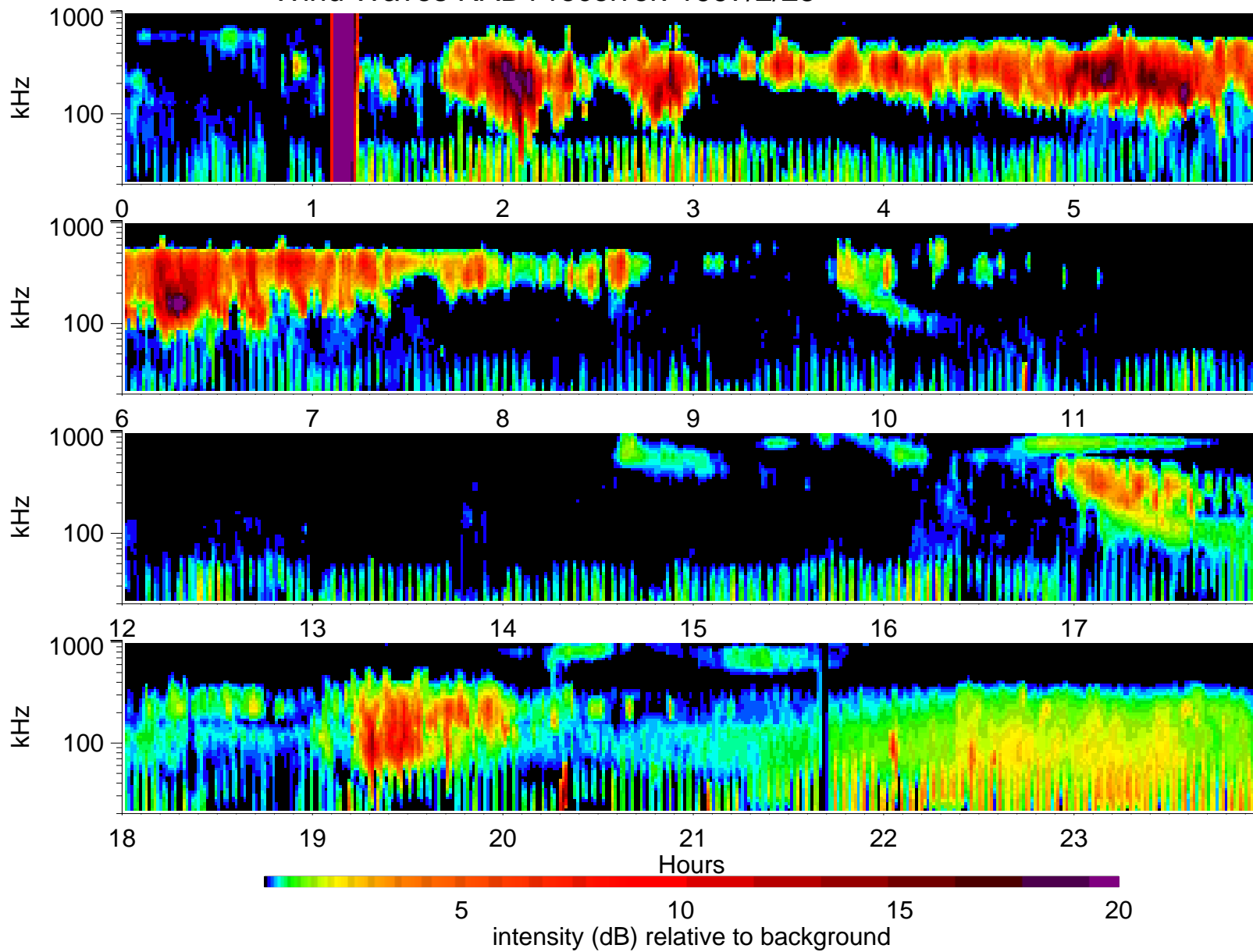
Wind Waves RAD1 receiver: 1997/2/25
