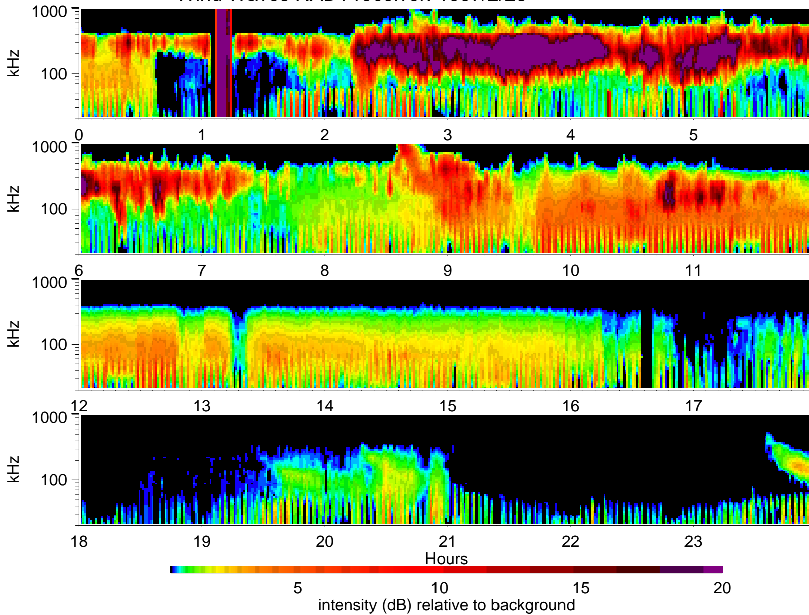
Wind Waves RAD1 receiver: 1997/2/23
