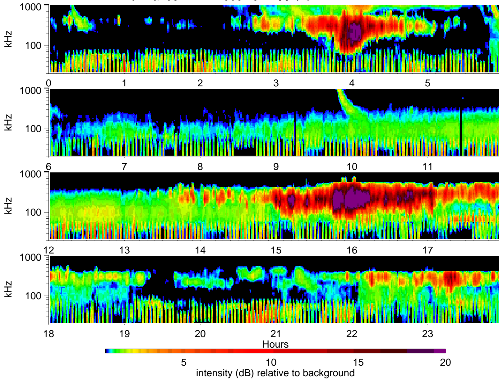
Wind Waves RAD1 receiver: 1997/2/22
