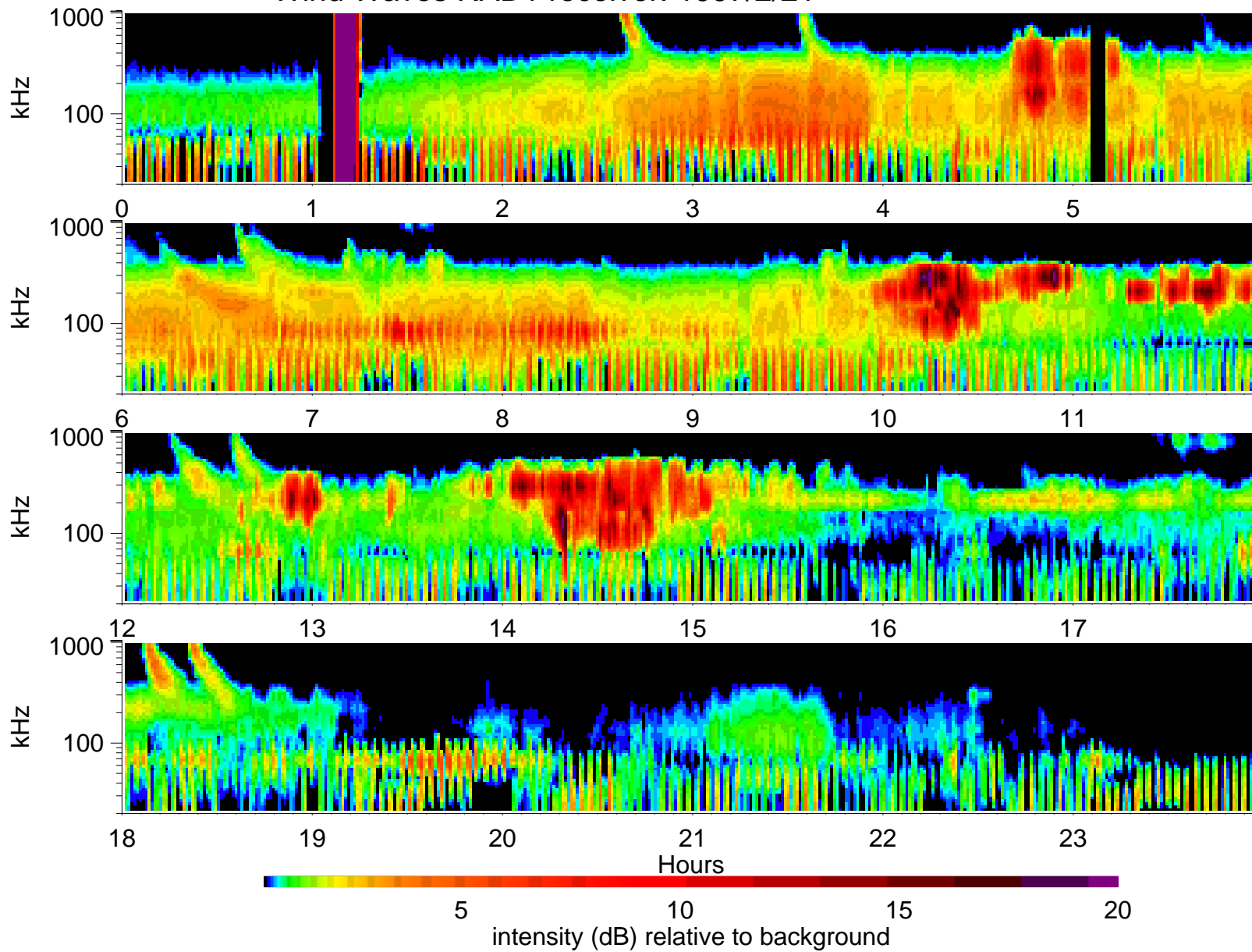
Wind Waves RAD1 receiver: 1997/2/21
