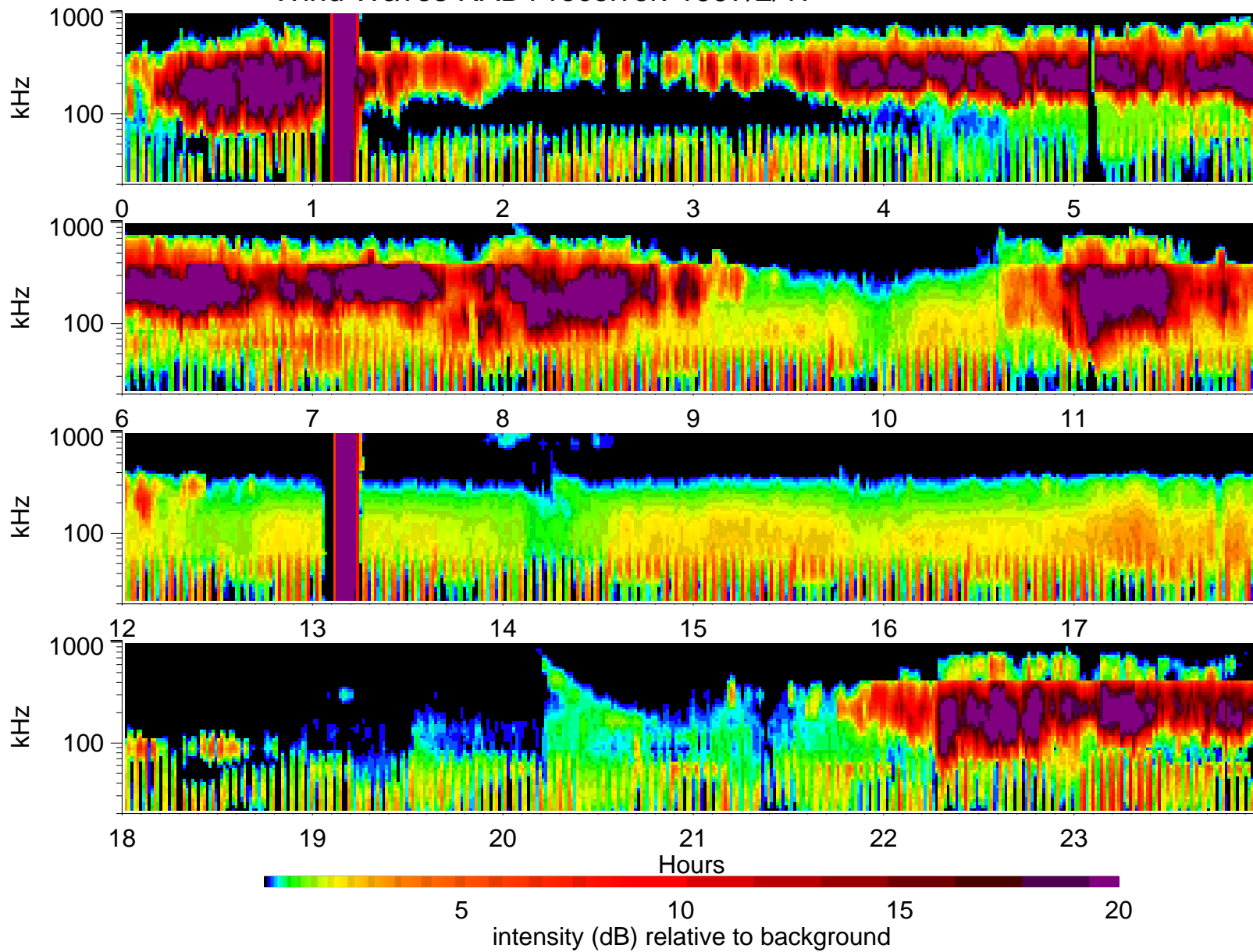
Wind Waves RAD1 receiver: 1997/2/17
