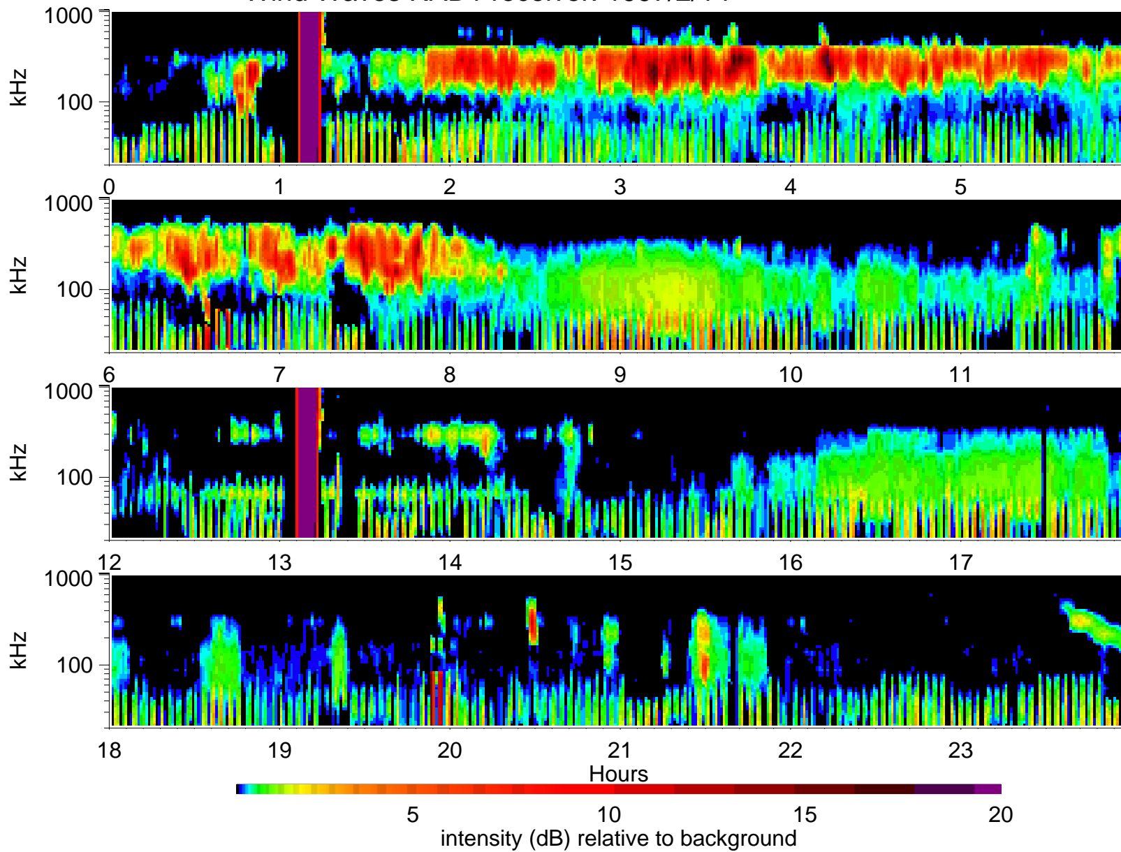
Wind Waves RAD1 receiver: 1997/2/14
