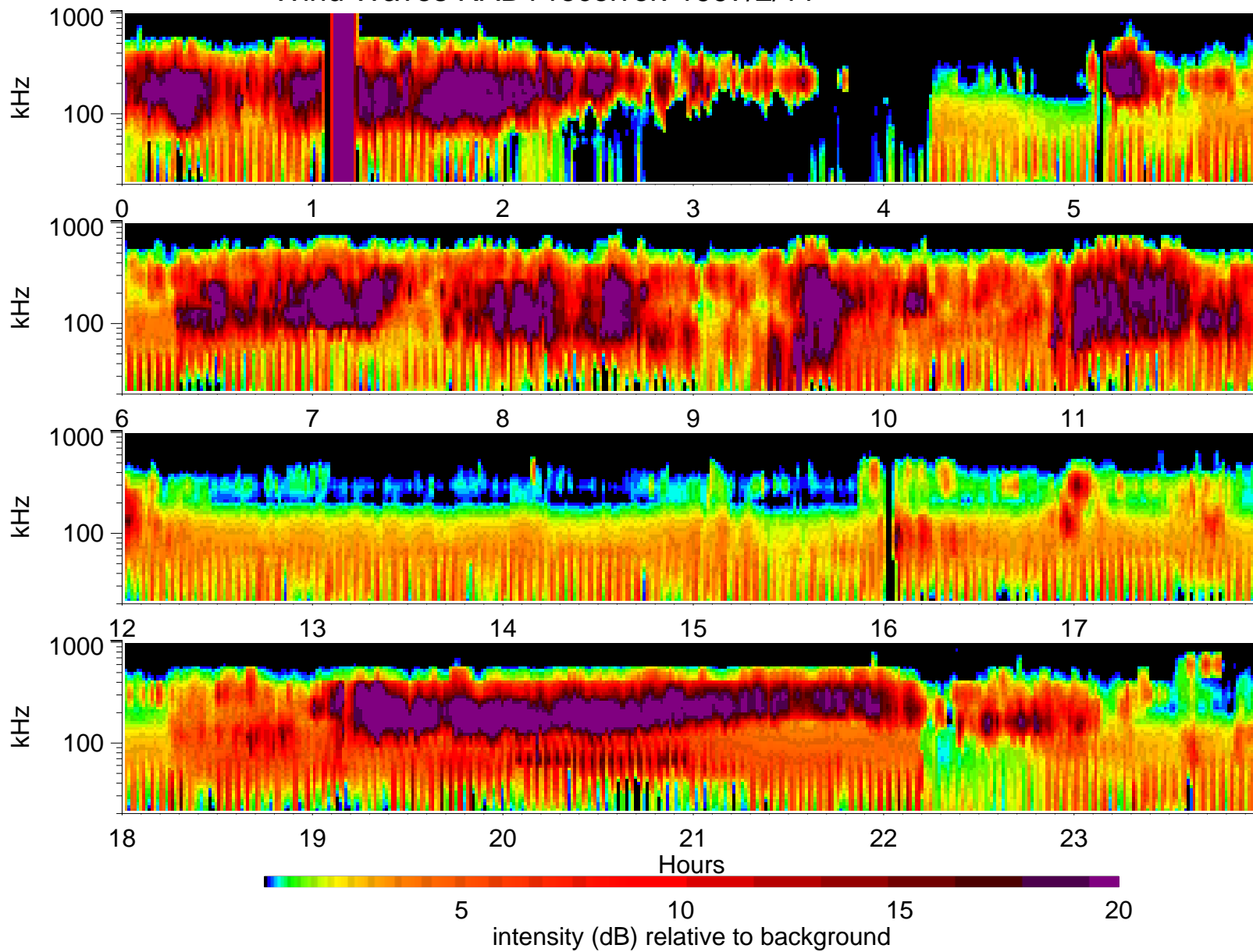
Wind Waves RAD1 receiver: 1997/2/11
