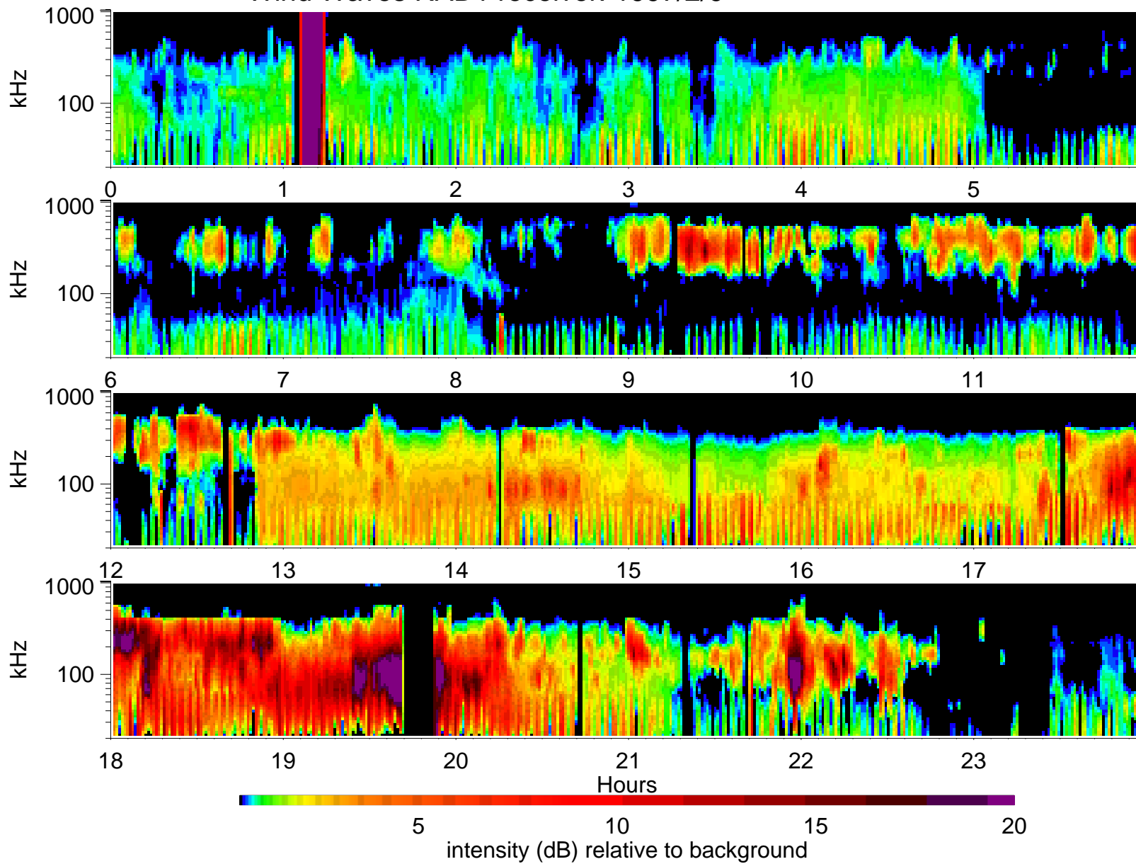
Wind Waves RAD1 receiver: 1997/2/9
