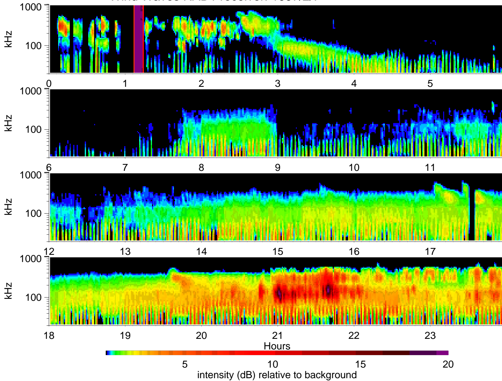
Wind Waves RAD1 receiver: 1997/2/7
