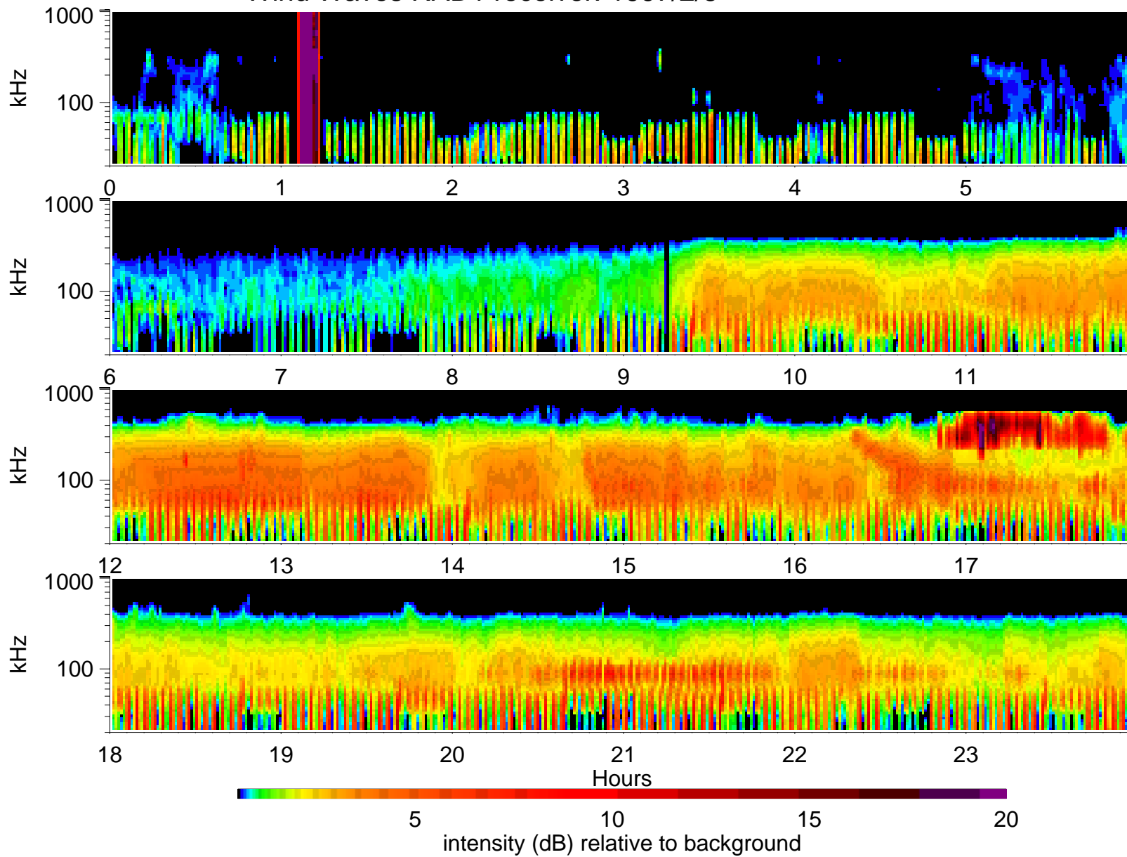
Wind Waves RAD1 receiver: 1997/2/5
