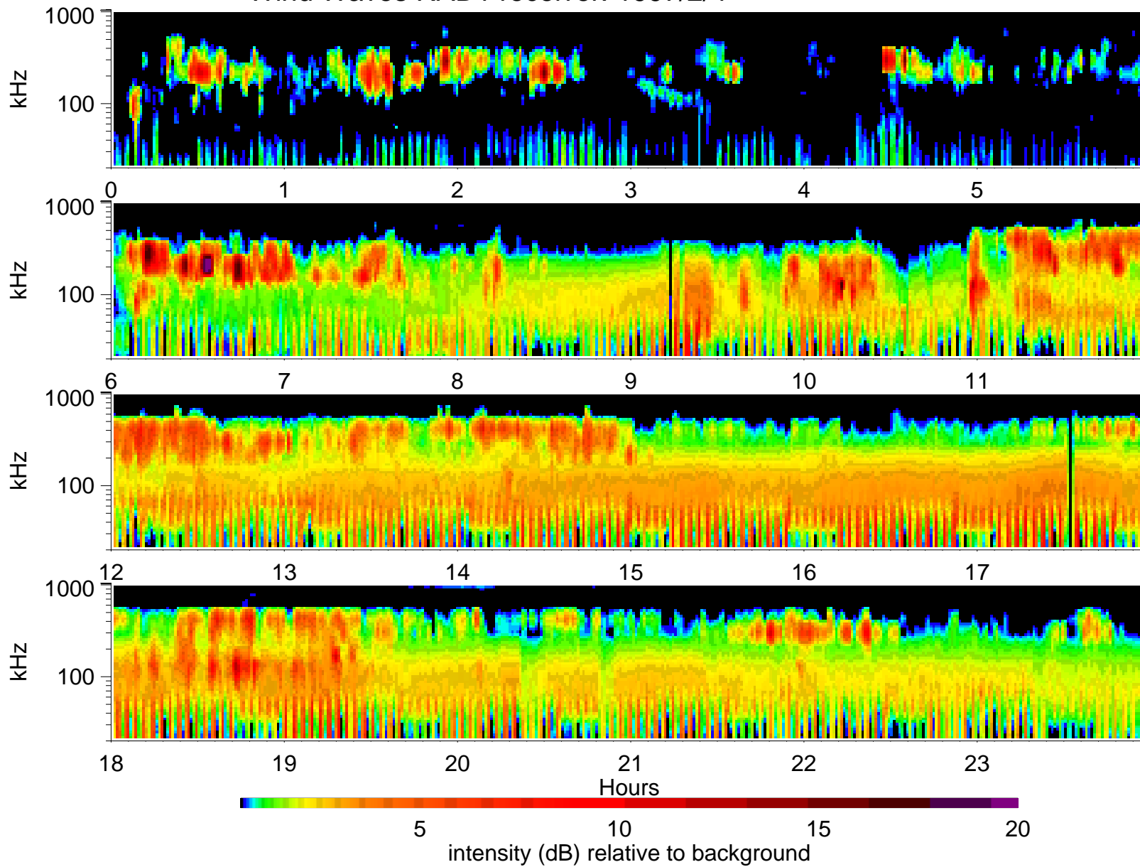
Wind Waves RAD1 receiver: 1997/2/4
