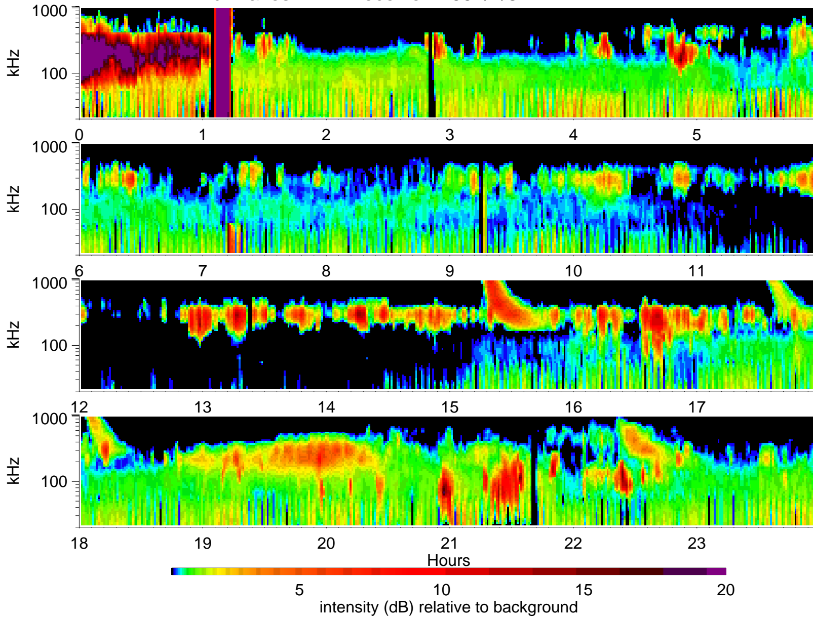
Wind Waves RAD1 receiver: 1997/2/3
