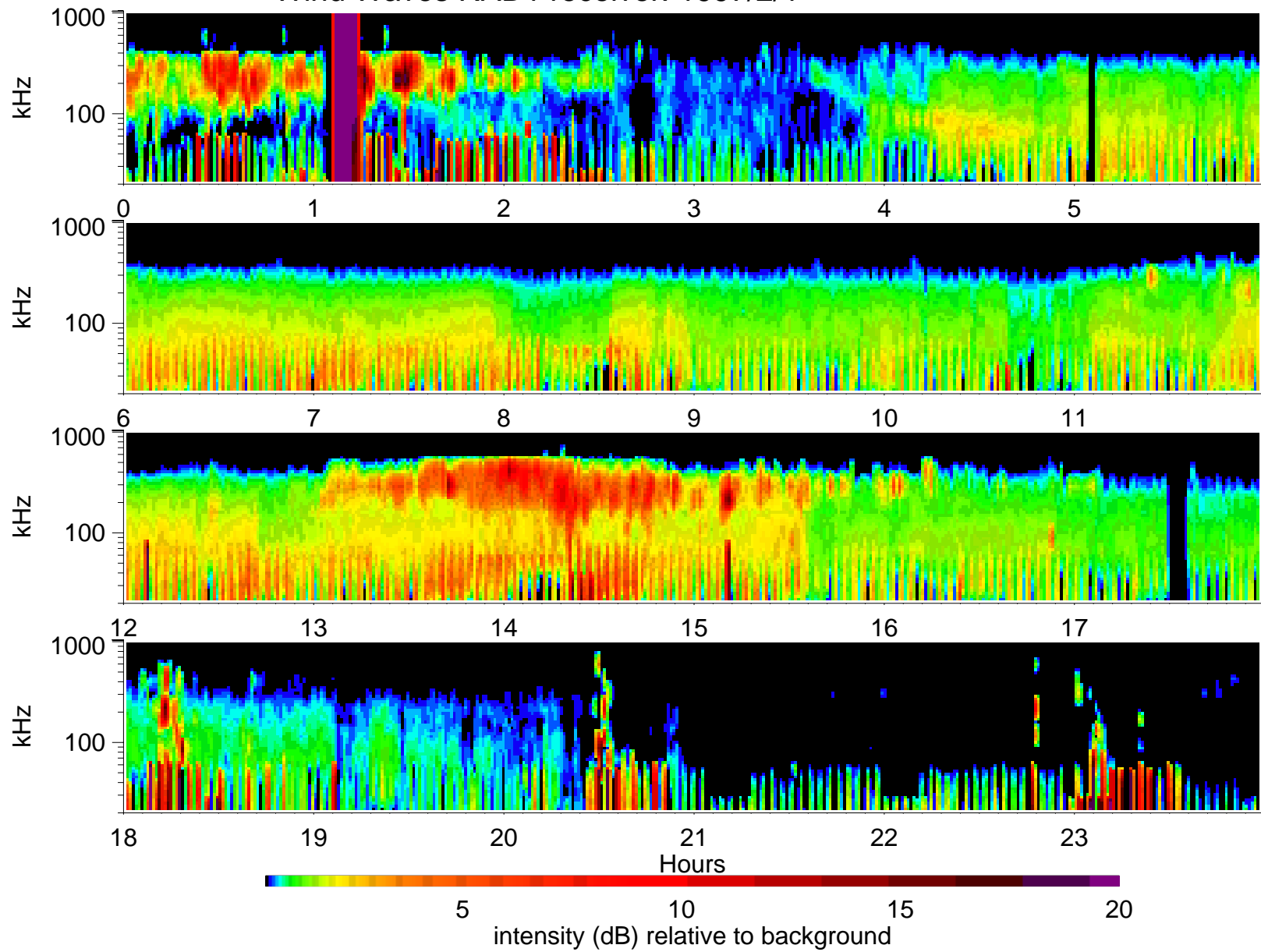
Wind Waves RAD1 receiver: 1997/2/1
