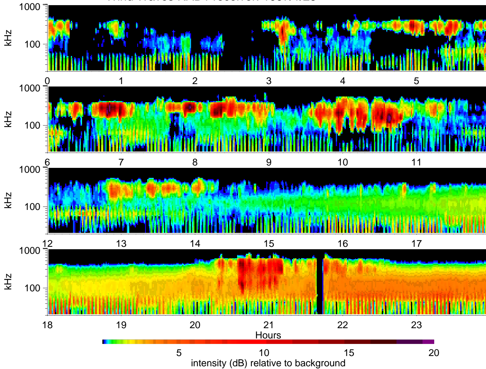
Wind Waves RAD1 receiver: 1997/1/25
