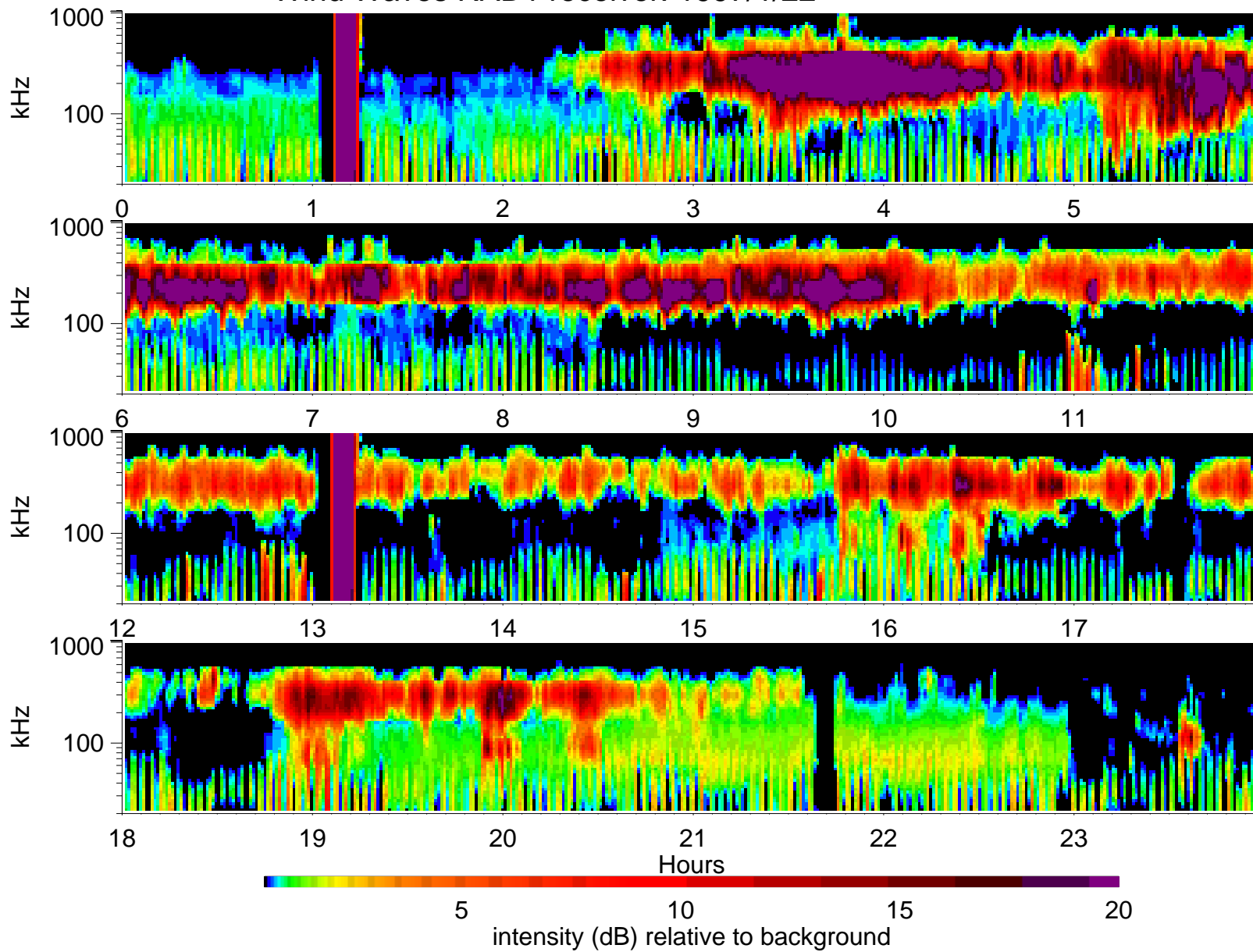
Wind Waves RAD1 receiver: 1997/1/22
