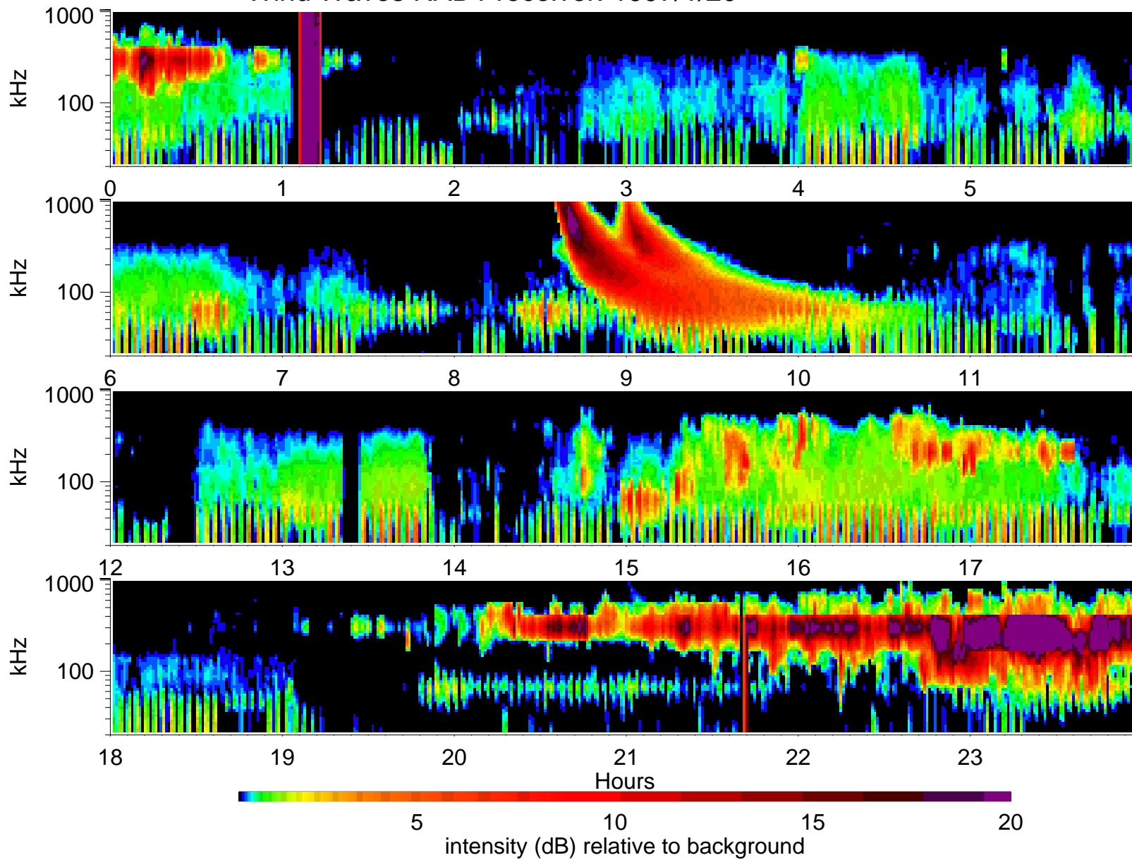
Wind Waves RAD1 receiver: 1997/1/20
