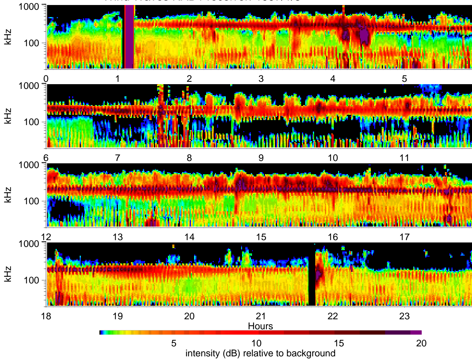
Wind Waves RAD1 receiver: 1997/1/8
