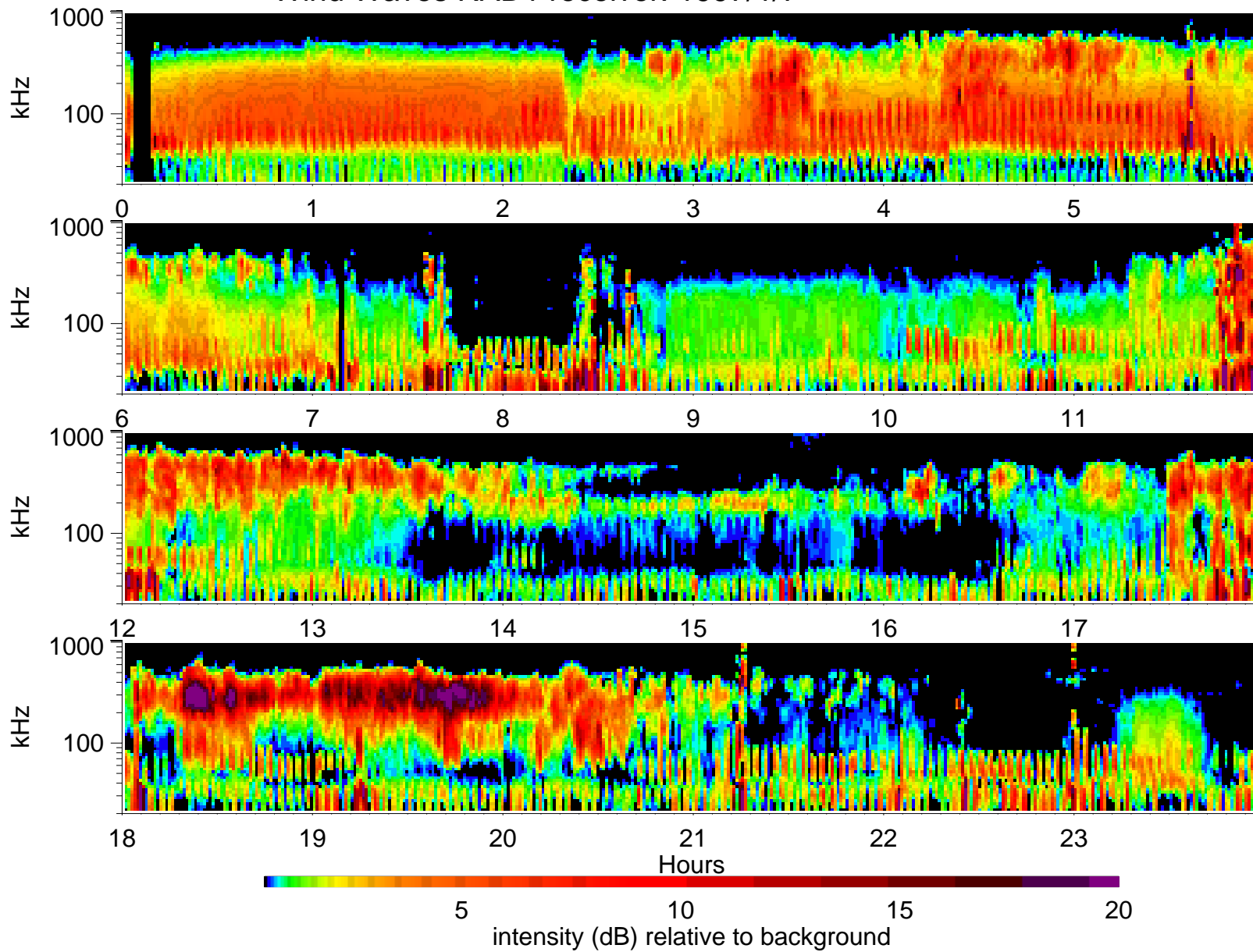
Wind Waves RAD1 receiver: 1997/1/7
