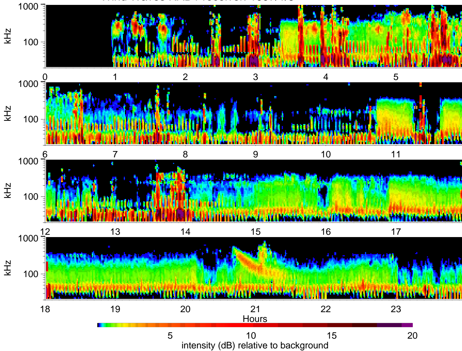
Wind Waves RAD1 receiver: 1997/1/5
