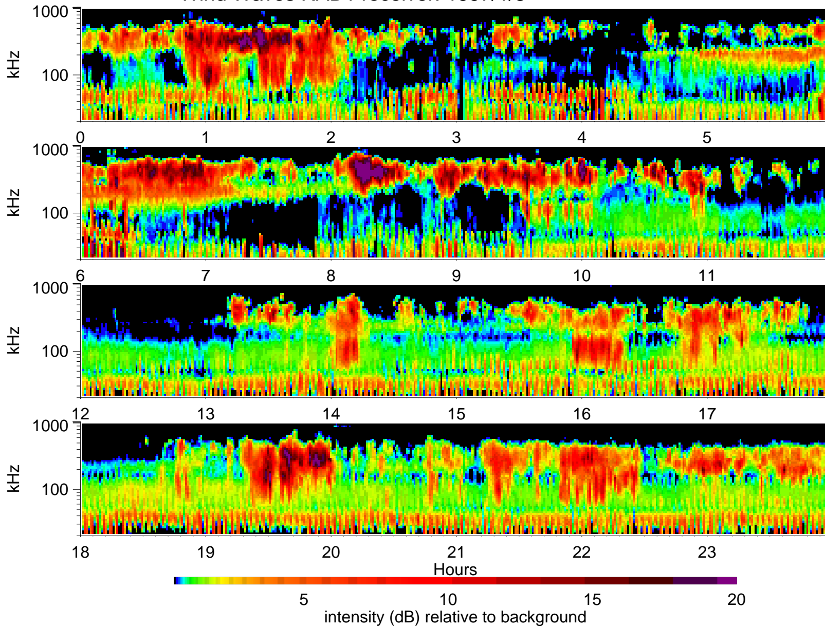
Wind Waves RAD1 receiver: 1997/1/3
