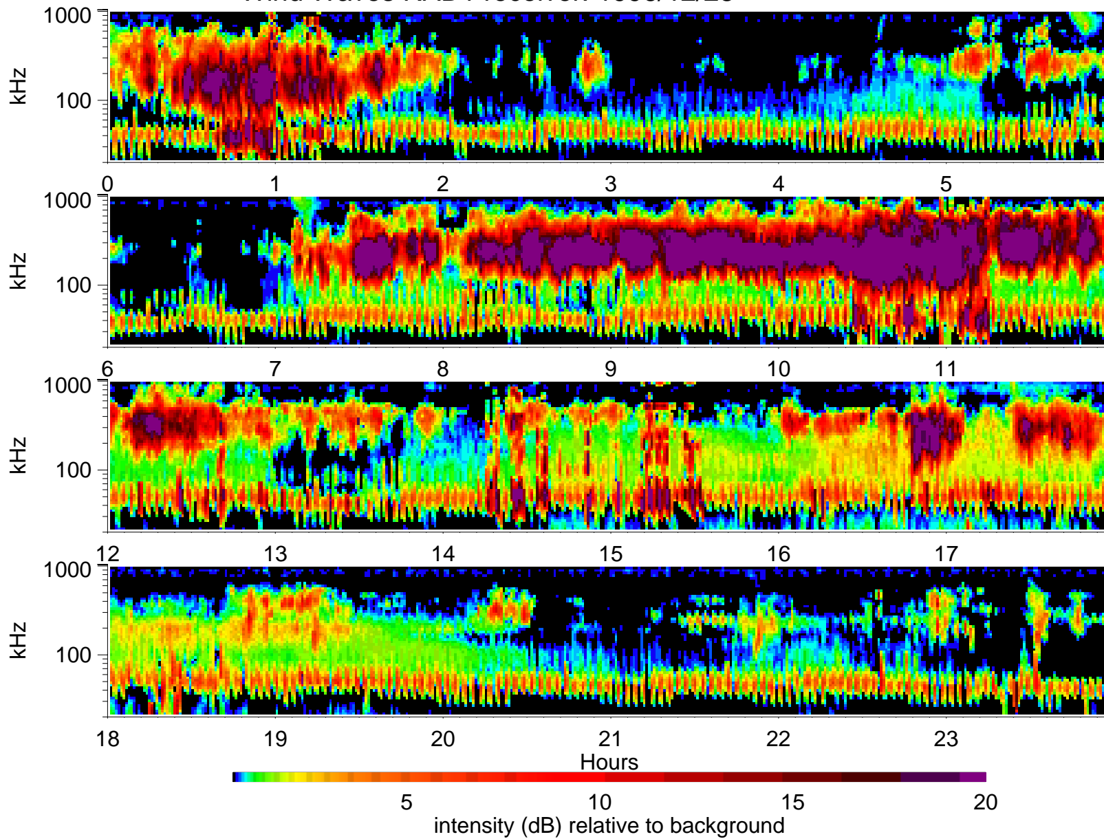
Wind Waves RAD1 receiver: 1996/12/28
