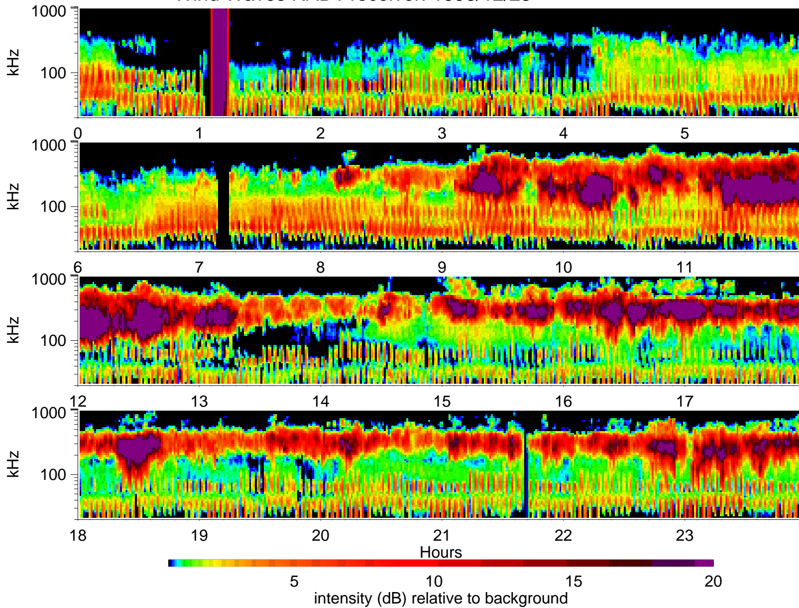
Wind Waves RAD1 receiver: 1996/12/25
