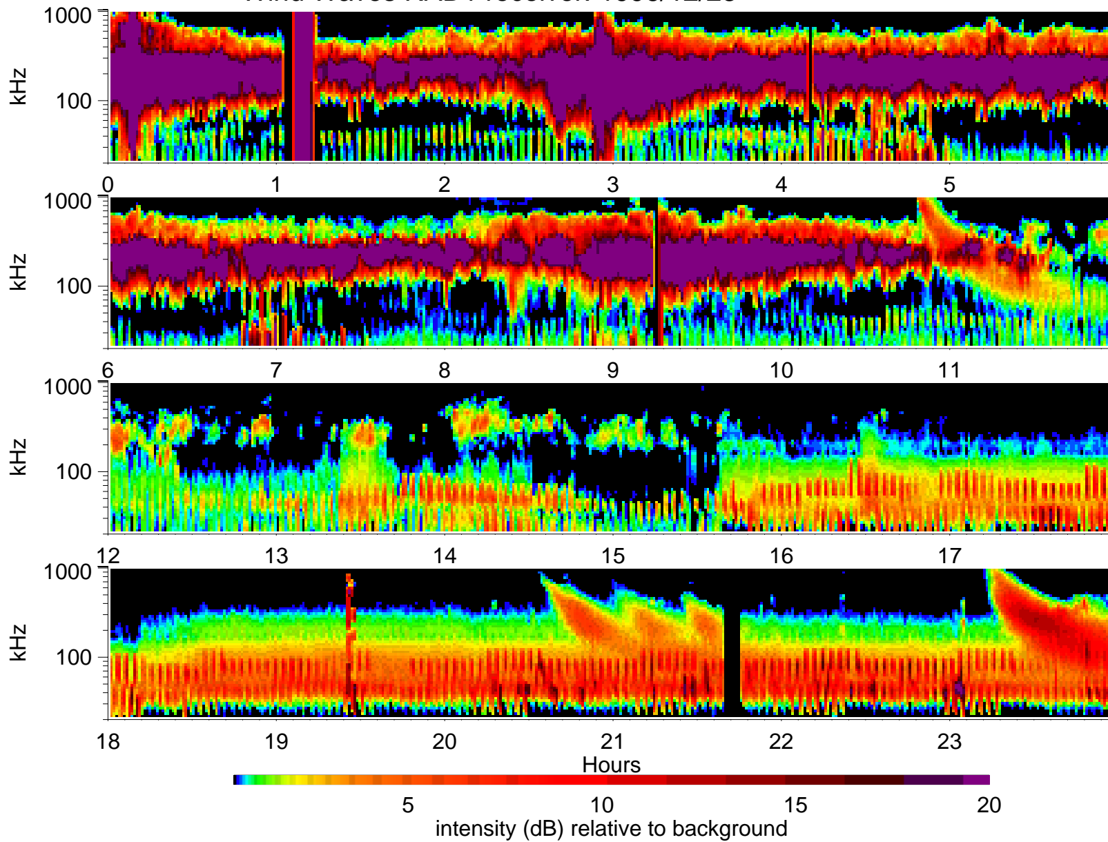
Wind Waves RAD1 receiver: 1996/12/23
