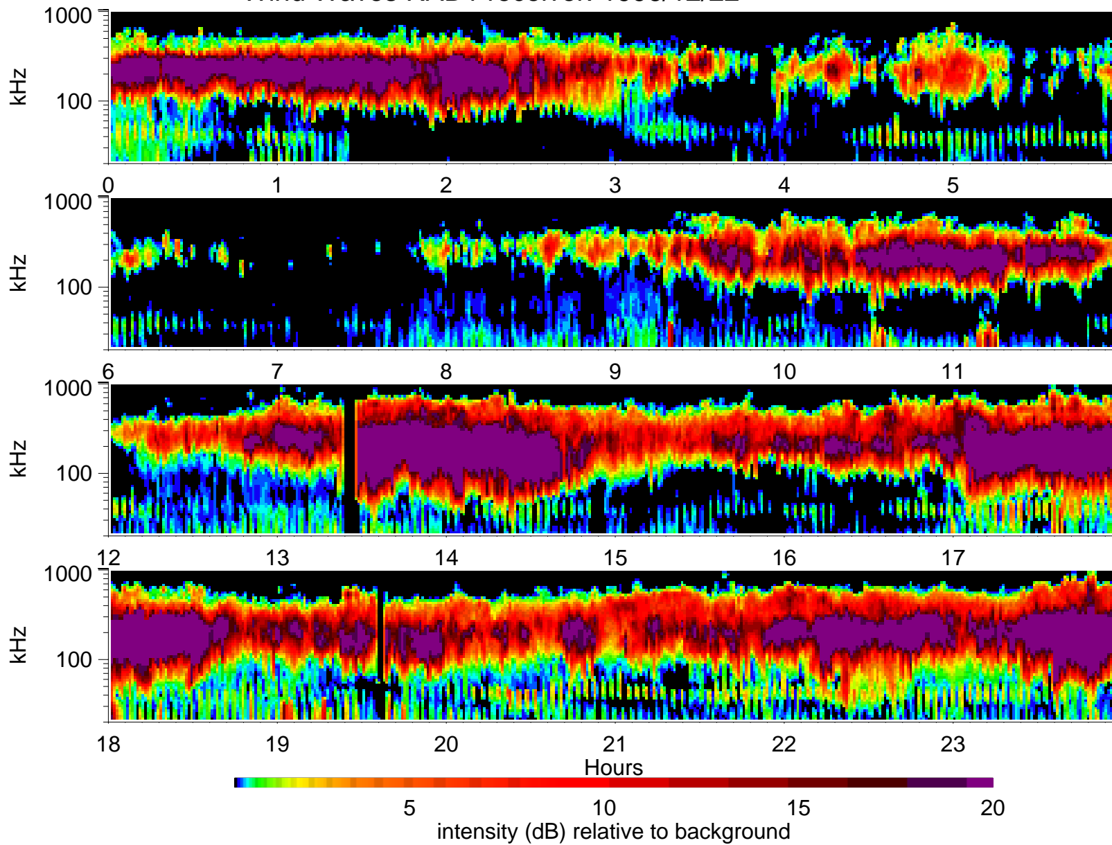
Wind Waves RAD1 receiver: 1996/12/22
