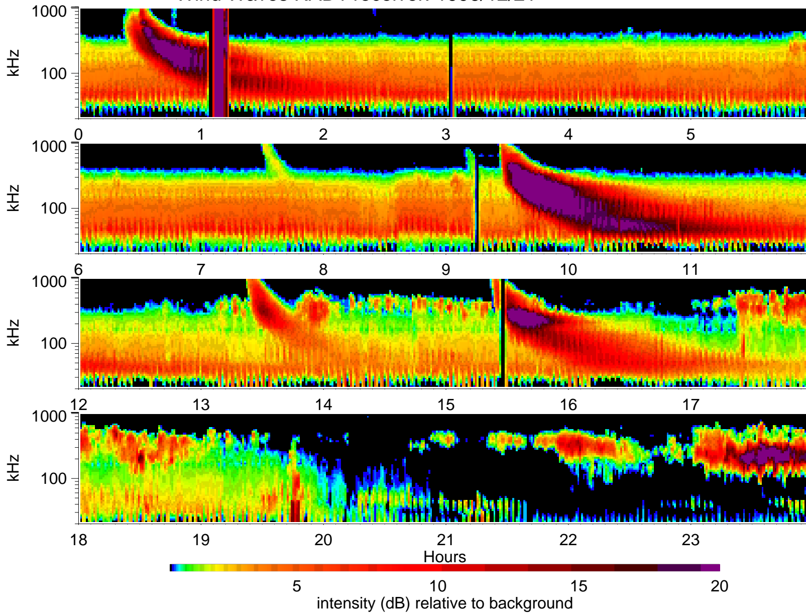
Wind Waves RAD1 receiver: 1996/12/21
