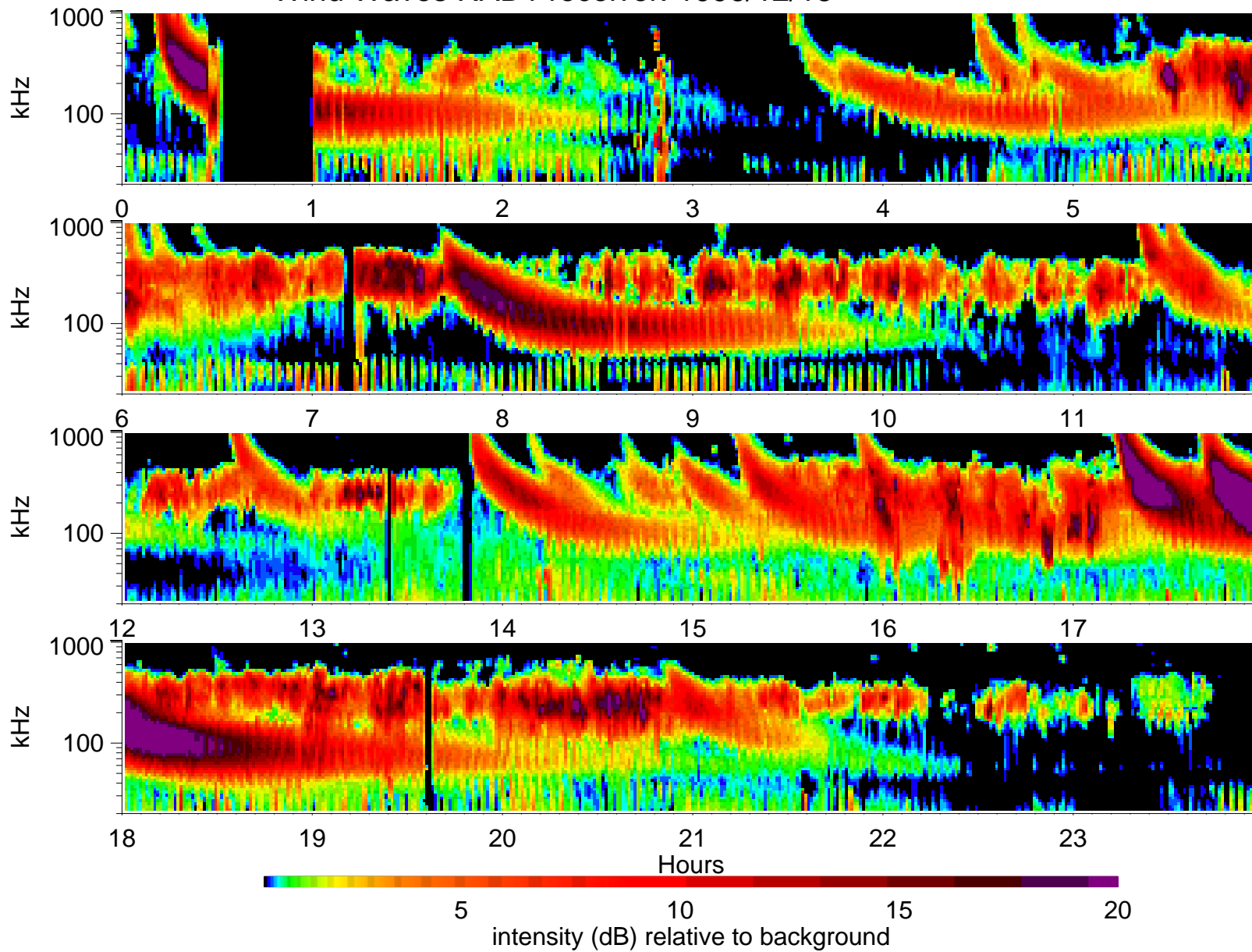
Wind Waves RAD1 receiver: 1996/12/18
